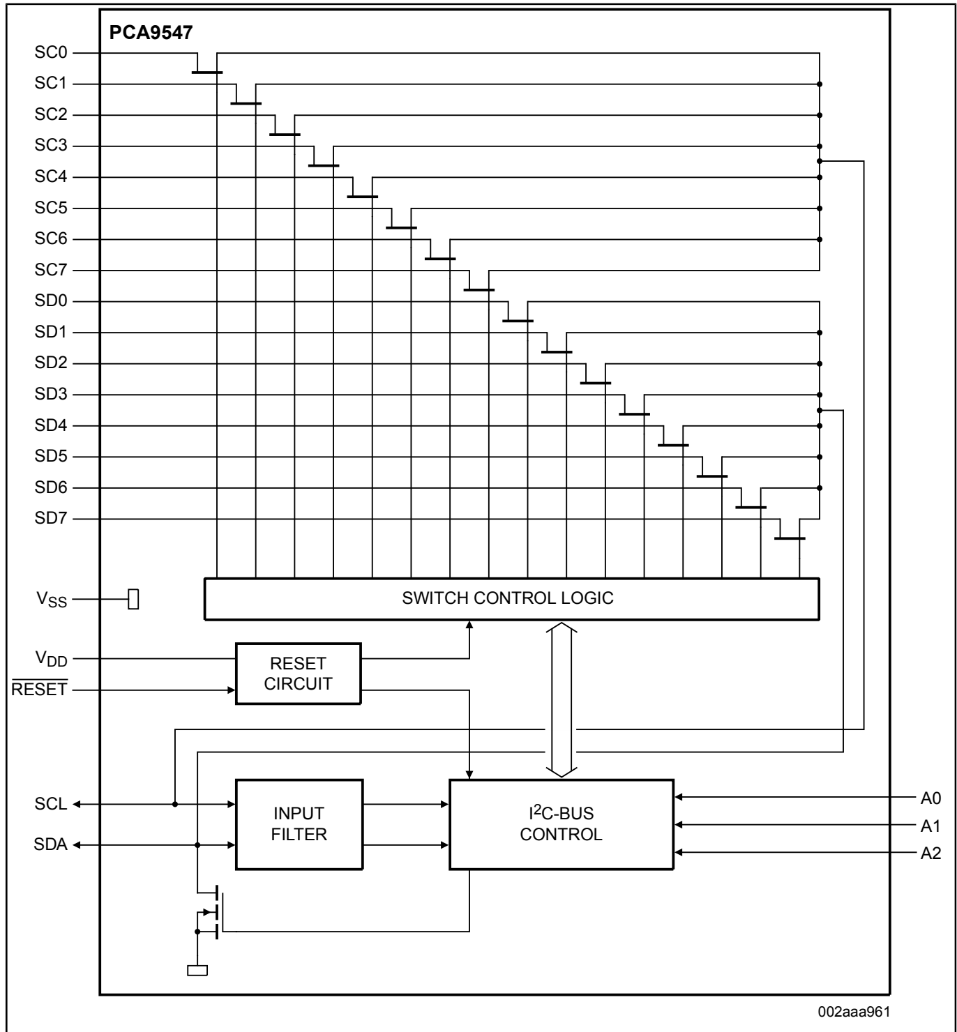
Block diagram: PCA9547BS, PCA9547D, PCA9547PW Block Diagram
