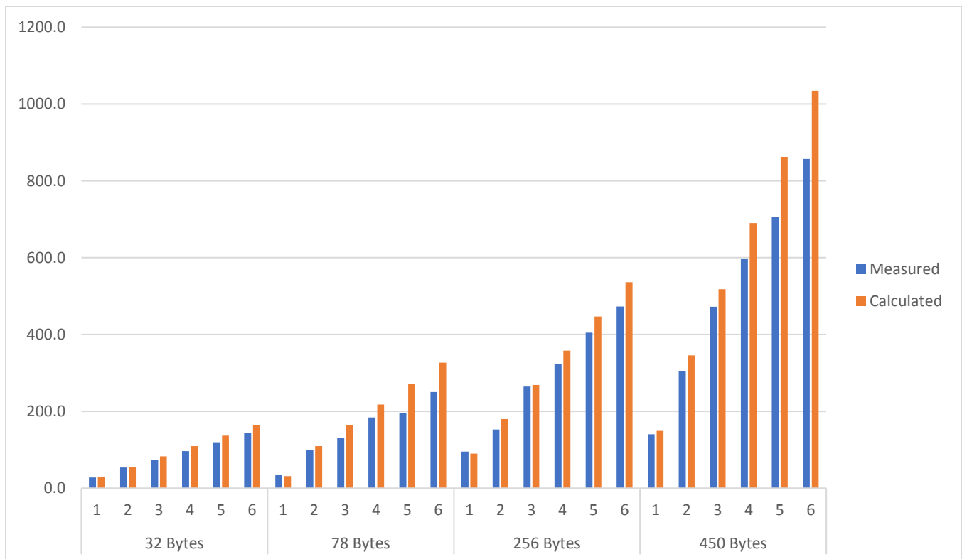
Figure 9. Calculated vs Measured RTT
