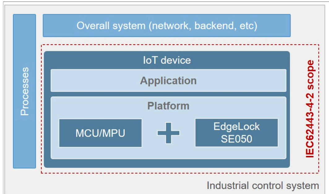
Figure 2. Breakdown of a simplified industrial control system
