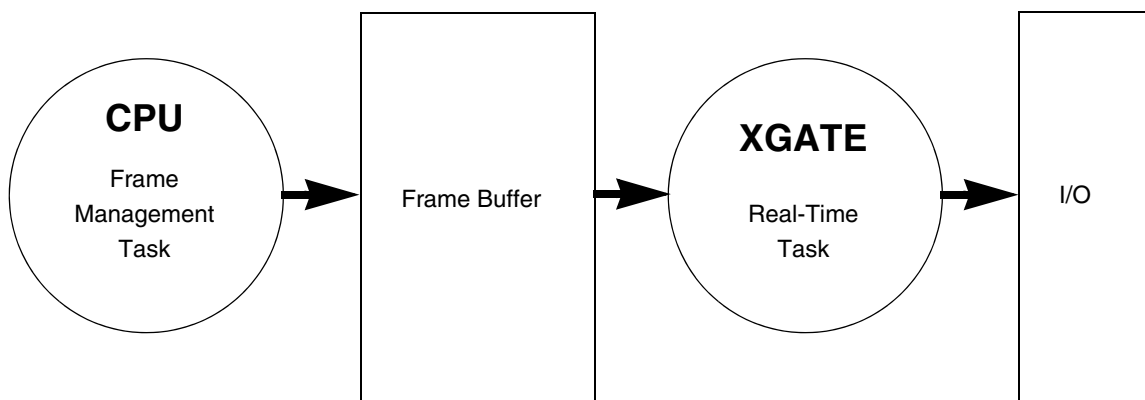
Figure 5. Software Architecture
