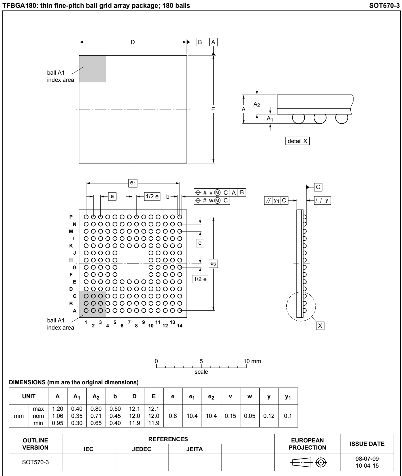
Fig. 1. Package outline TFBGA180 (SOT570-3)
