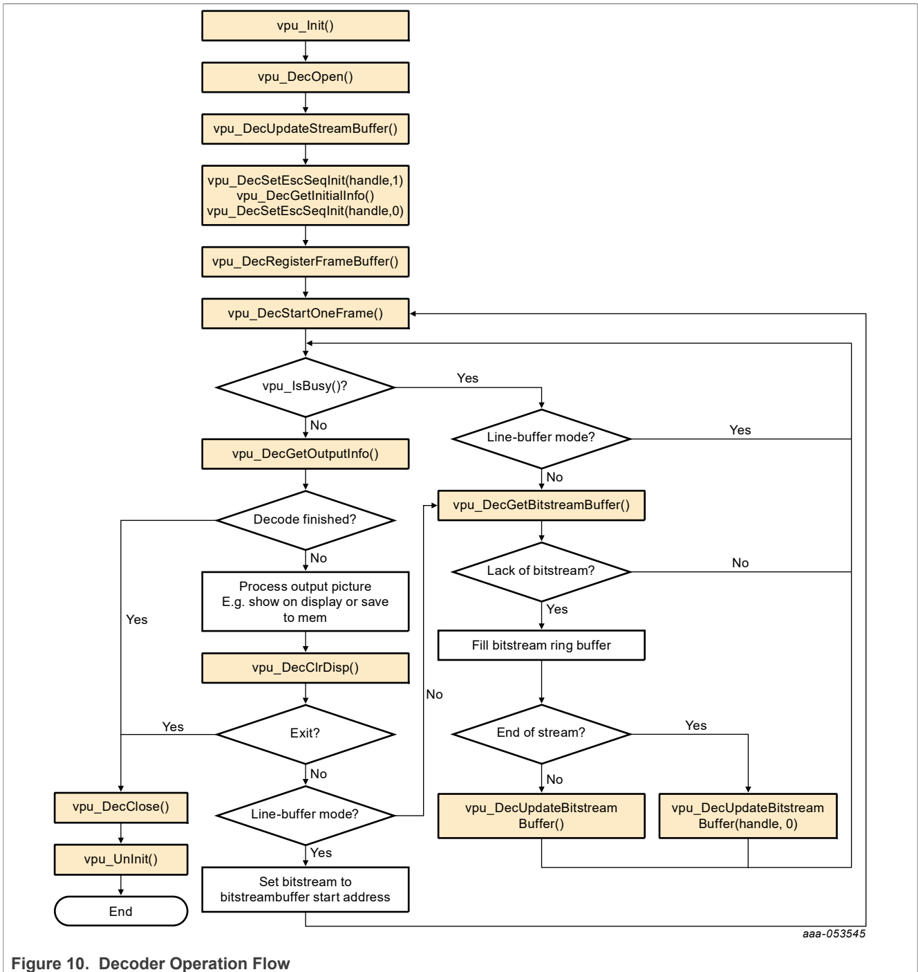
Figure 10. Decoder Operation Flow
