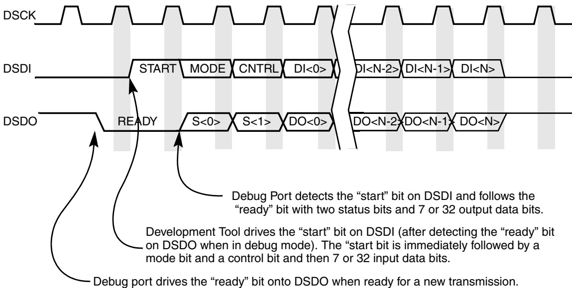
Figure 45-9. Asynchronous Clocked Serial Communications
