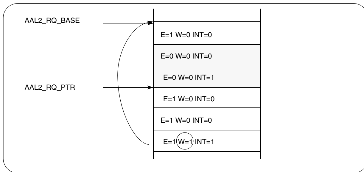
Figure 43-7. AAL2_Rx_Queue Example
