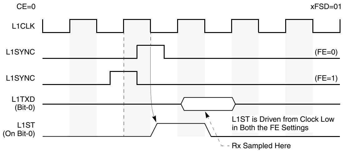
Figure 20-17. Falling Edge (FE) Affect When CE = 0 and xFSD = 01
