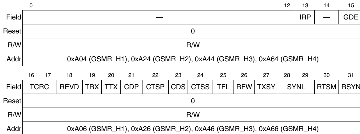
Figure 21-2. GSMR_H—General SCC Mode Register (High Order)
