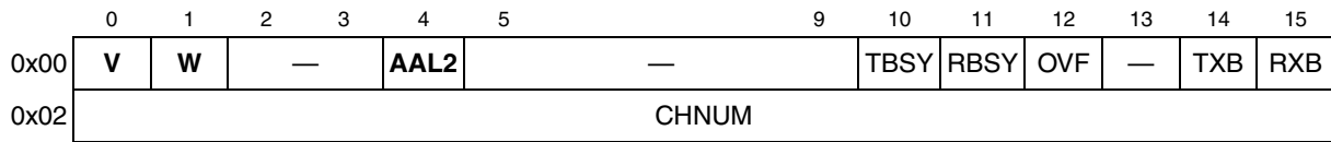
Figure 43-12. AAL2-Specific Exception Entry Format
