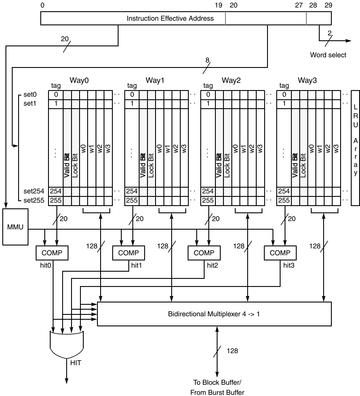
Figure 7-1. MPC862P Instruction Cache Organization
