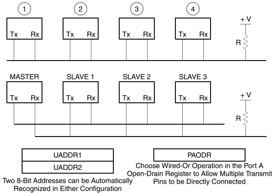
Figure 22-2. Two UART Multidrop Configurations
