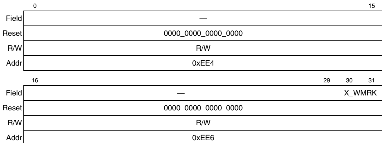
Figure 44-20. X_WMRK Register
