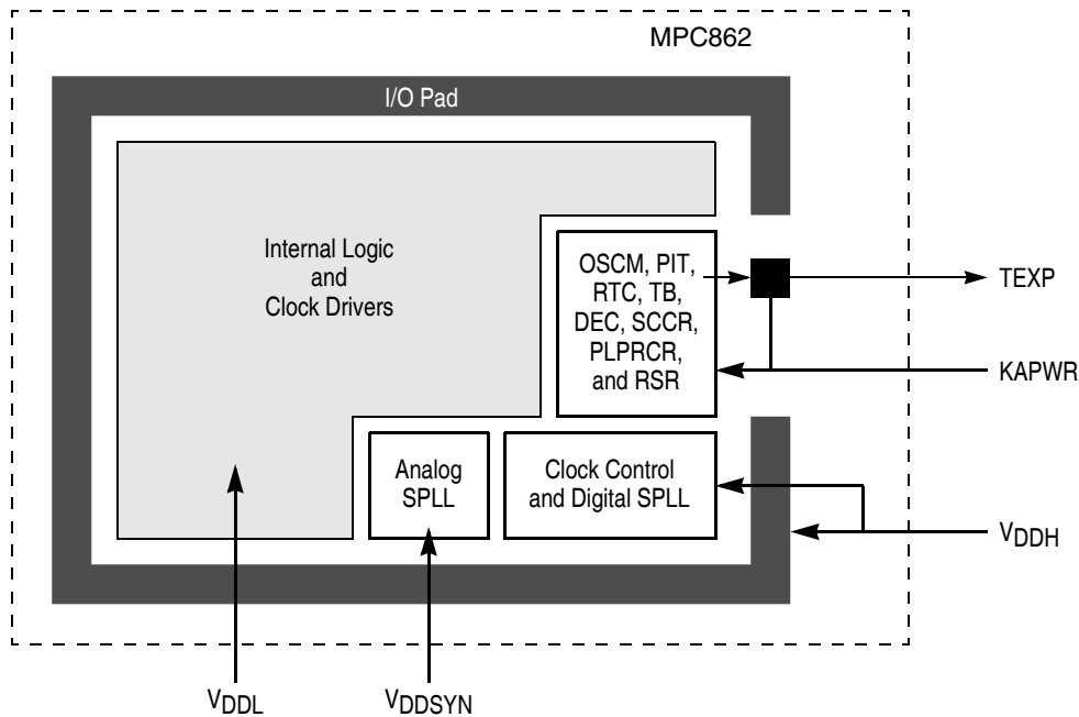
Figure 14-12. MPC862 Power Rails
