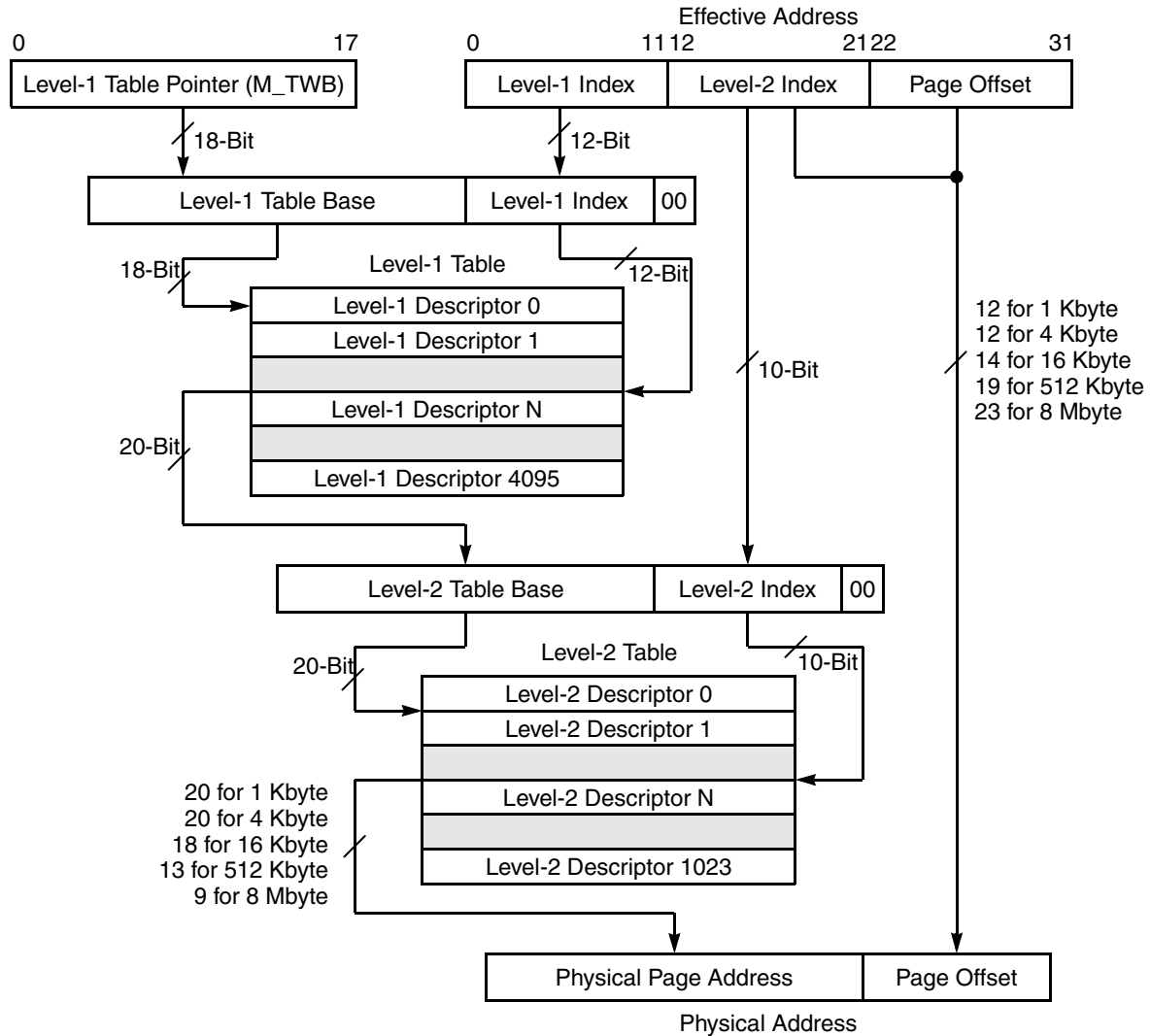
Figure 8-5. Two-Level Translation Table (MD_CTR[TWAM] = 0)
