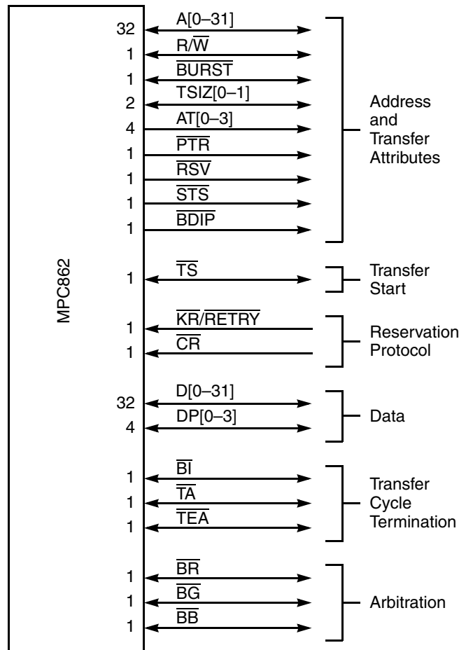
Figure 13-2. MPC862 Bus Signals
