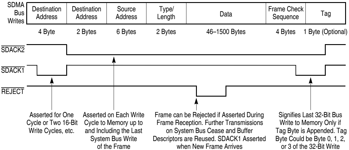
Figure 27-5. MPC862 Ethernet Parallel CAM Interface
