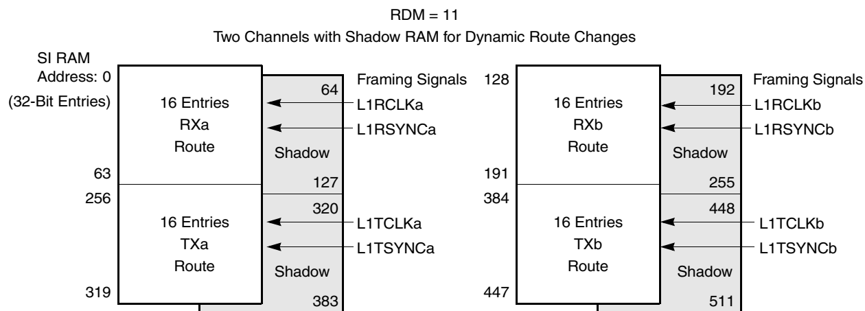
Figure 20-9. SI RAM Partitioning Using Two TDMs with Dynamic Frames
