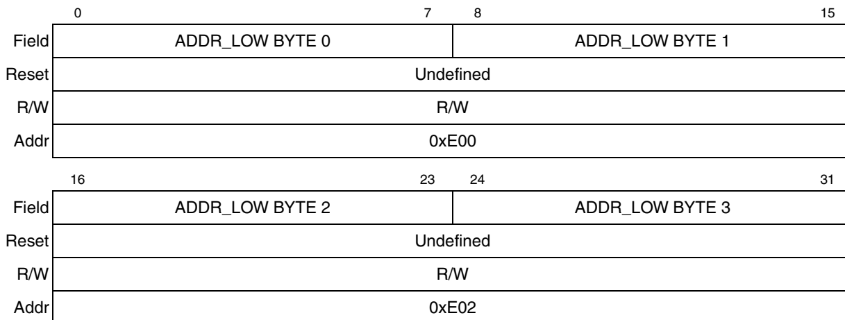
Figure 44-4. ADDR_LOW Register
