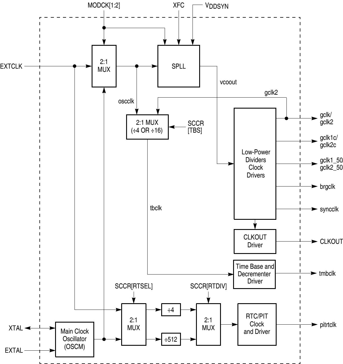
Figure 14-1. Clock Source and Distribution
