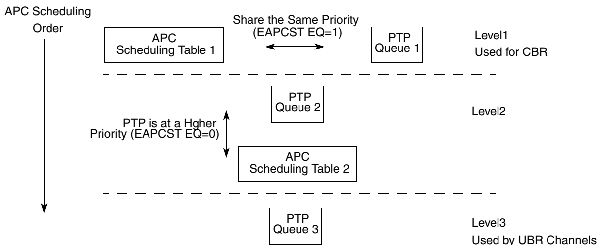
Figure 39-9. Example of Three APC Priority Levels Combining APC Scheduling Tables and APC PTP Queues
