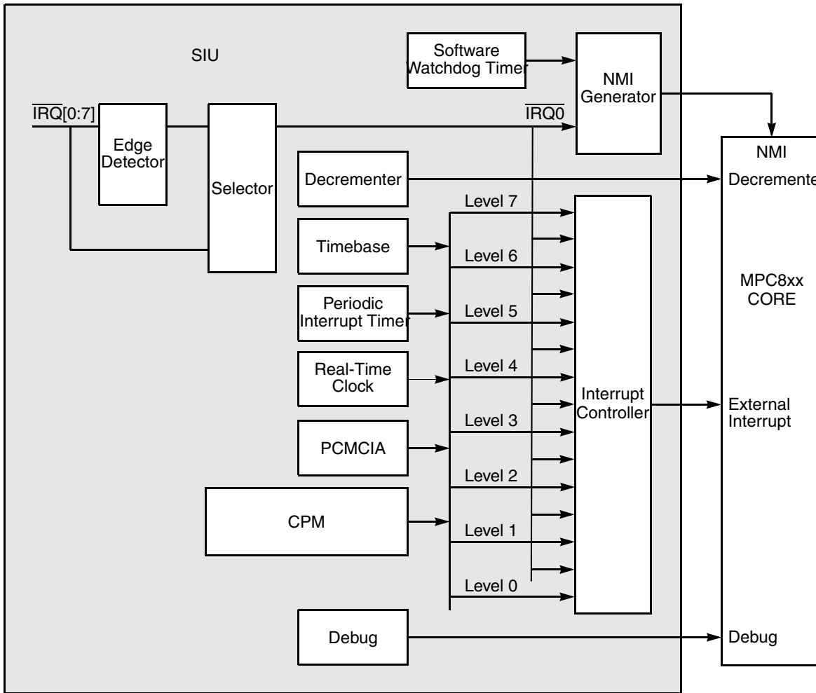
Figure 10-7. MPC862 Interrupt Structure
