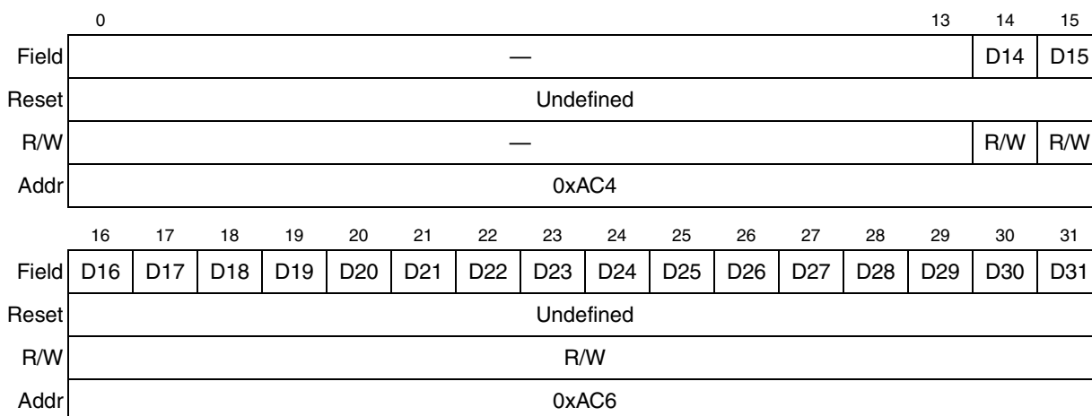
Figure 33-8. Port B Data Register (PBDAT)
