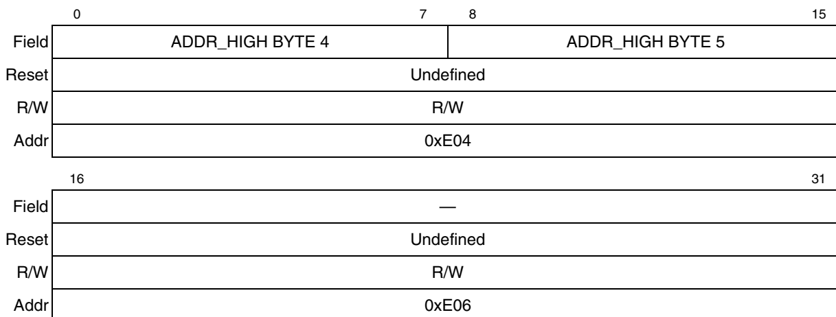
Figure 44-5. ADDR_HIGH Register
