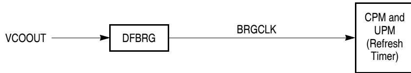
Figure 14-10. BRGCLK Divider
