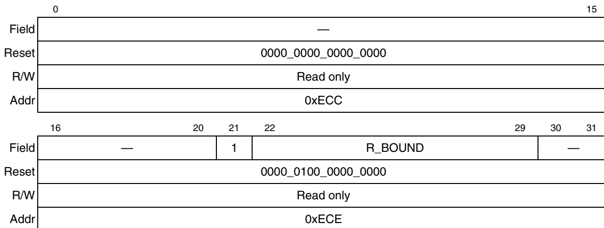
Figure 44-18. R_BOUND Register
