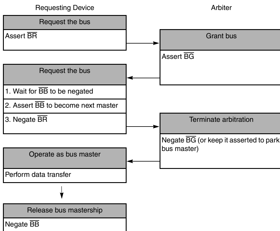
Figure 13-21. Basic Bus Arbitration Protocol
