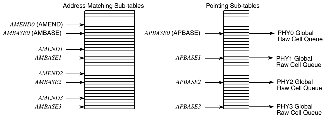
Figure 38-13. Address Mapping Tables for Internal Channels in Multi-PHY Operation
