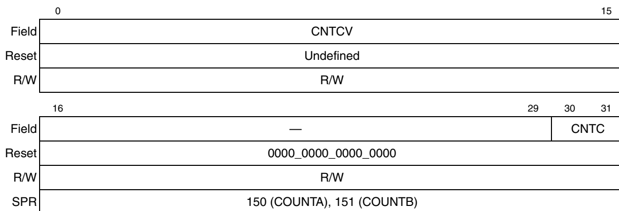
Figure 45-21. Breakpoint Counter Value and Control Registers (COUNTA/COUNTB)
