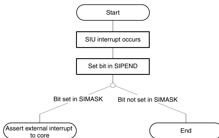
Figure 10-8. SIU Interrupt Processing
