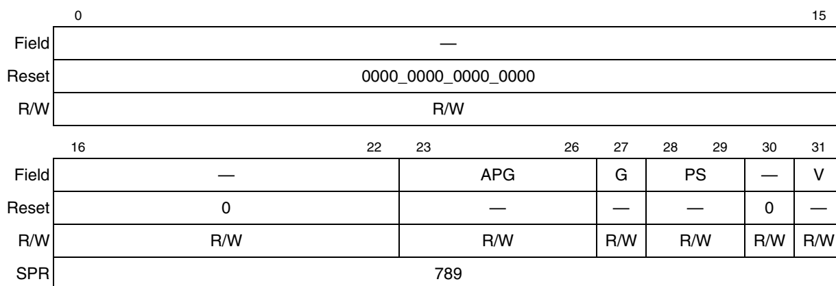
Figure 8-9. IMMU Tablewalk Control Register (MI_TWC)
