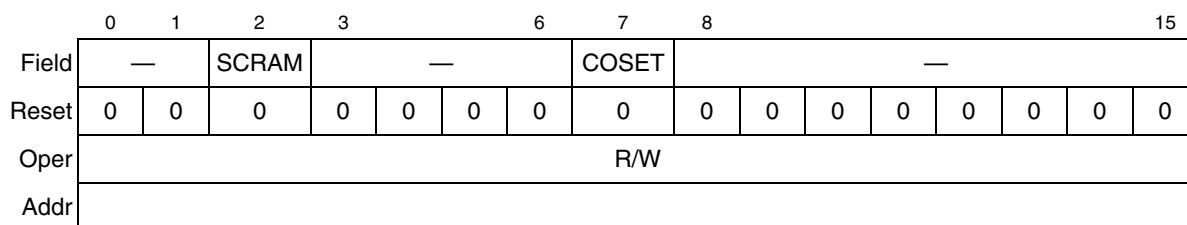
Figure 41-3. Serial ATM Mode Register (PSMR)
