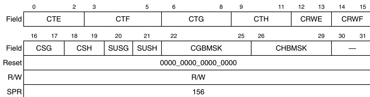
Figure 45-19. Load/Store Support Comparators Control Register (LCTRL1)
