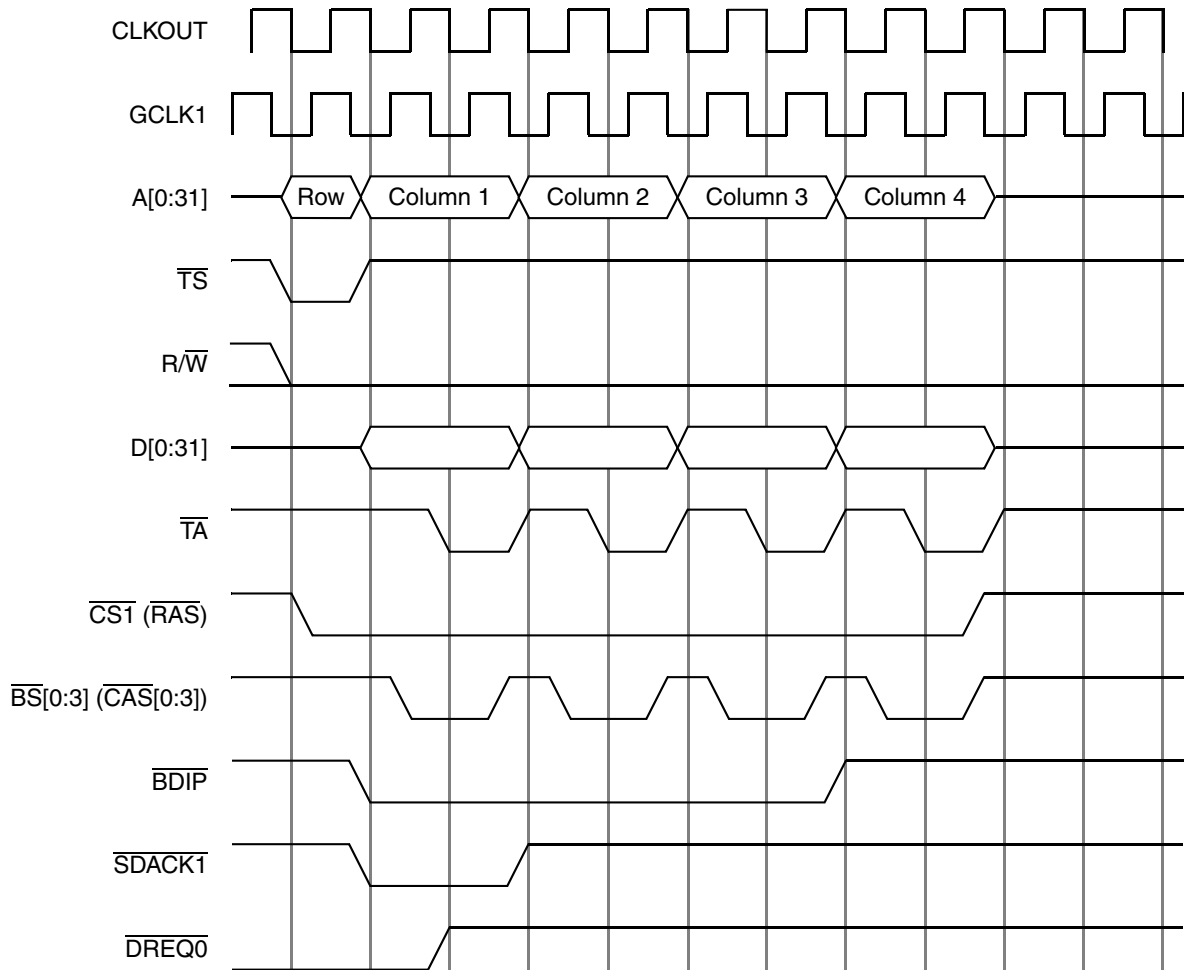
Figure 19-15. Single-Address IDMA1 Burst Timing (Single-Buffer Mode)
