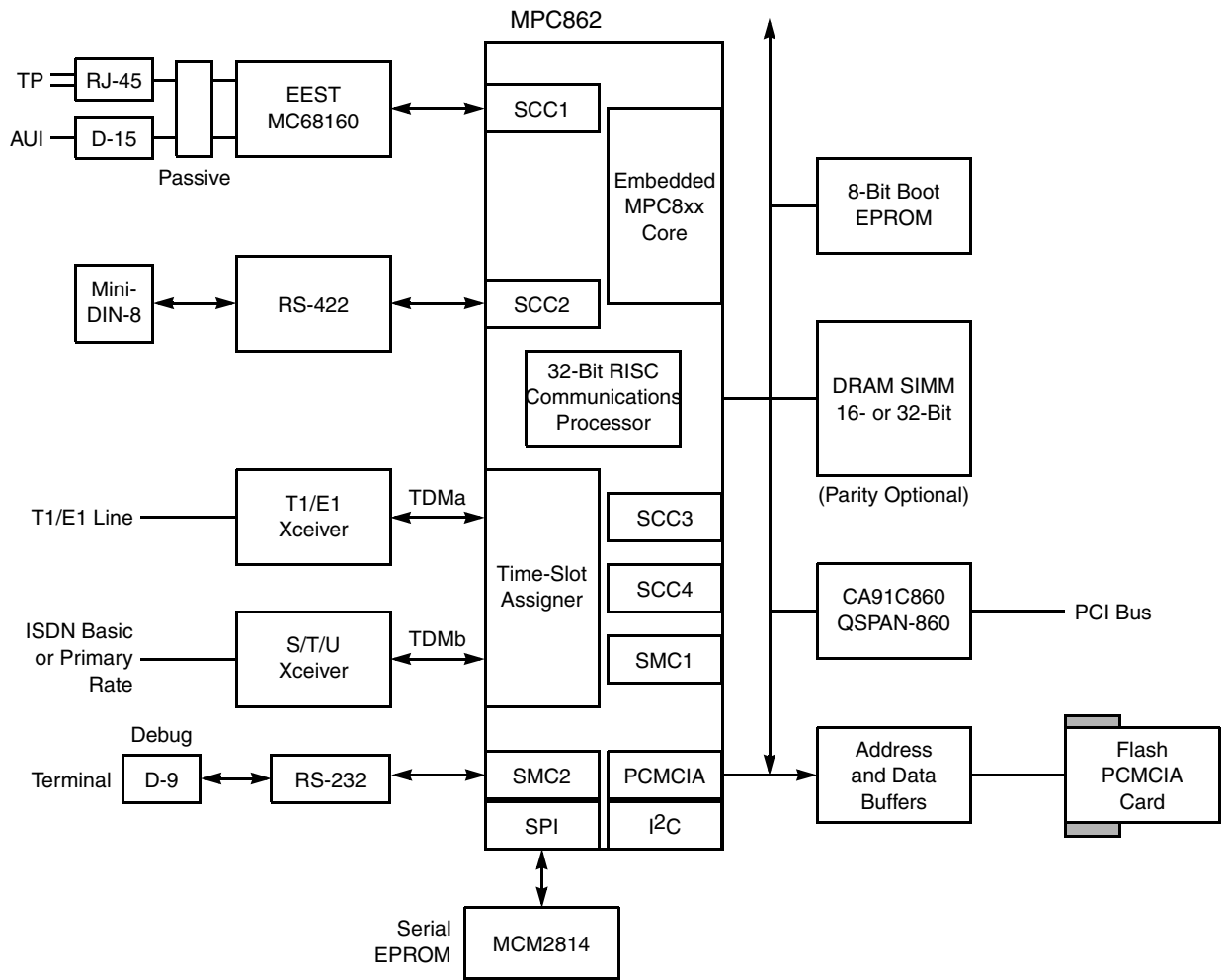
Figure 17-2. MPC862 Application Design Example
