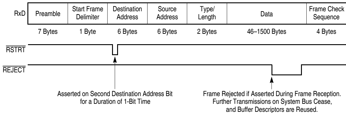
Figure 27-4. MPC862 Ethernet Serial CAM Interface
