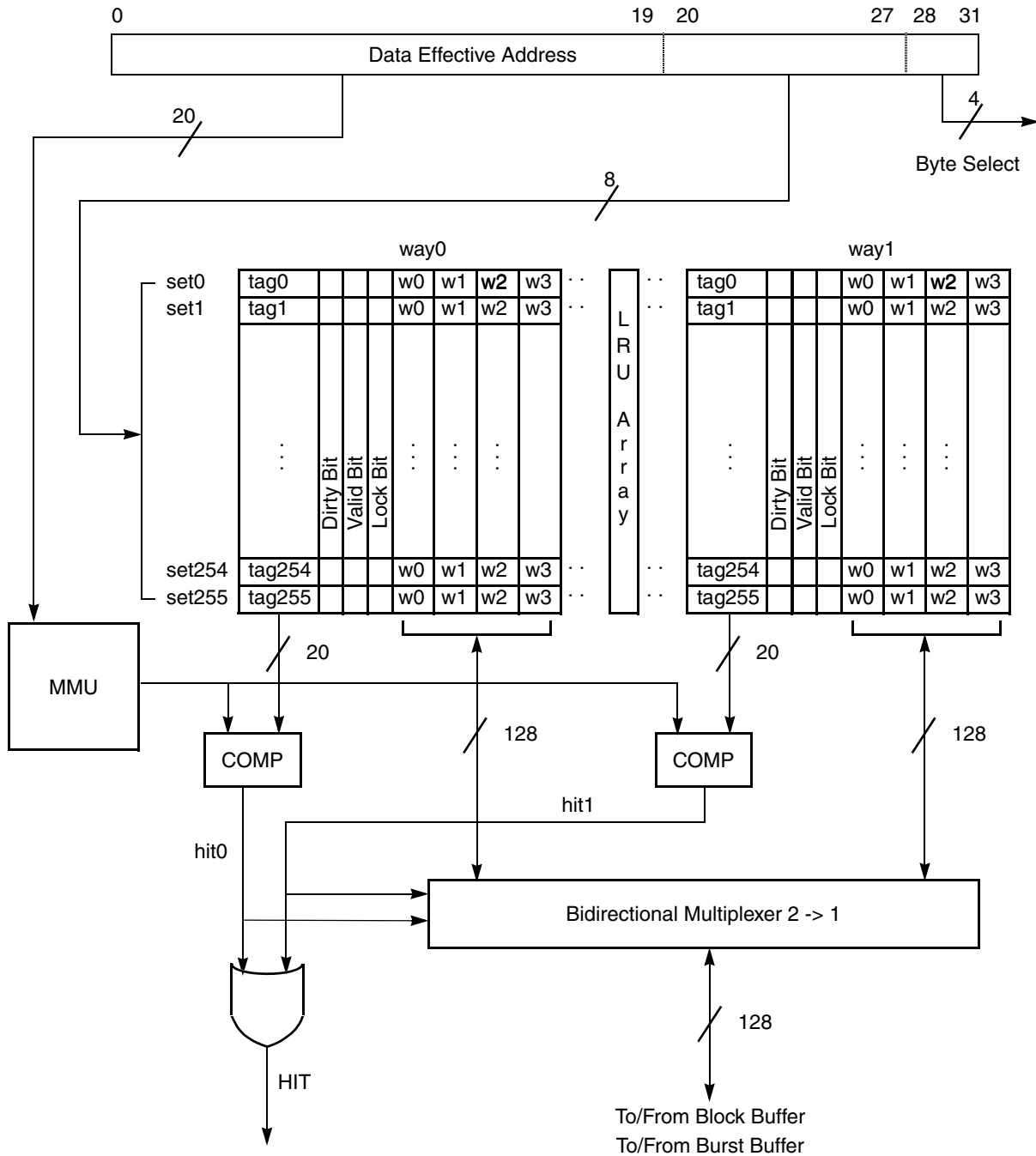
Figure 7-3. MPC862P Data Cache Organization
