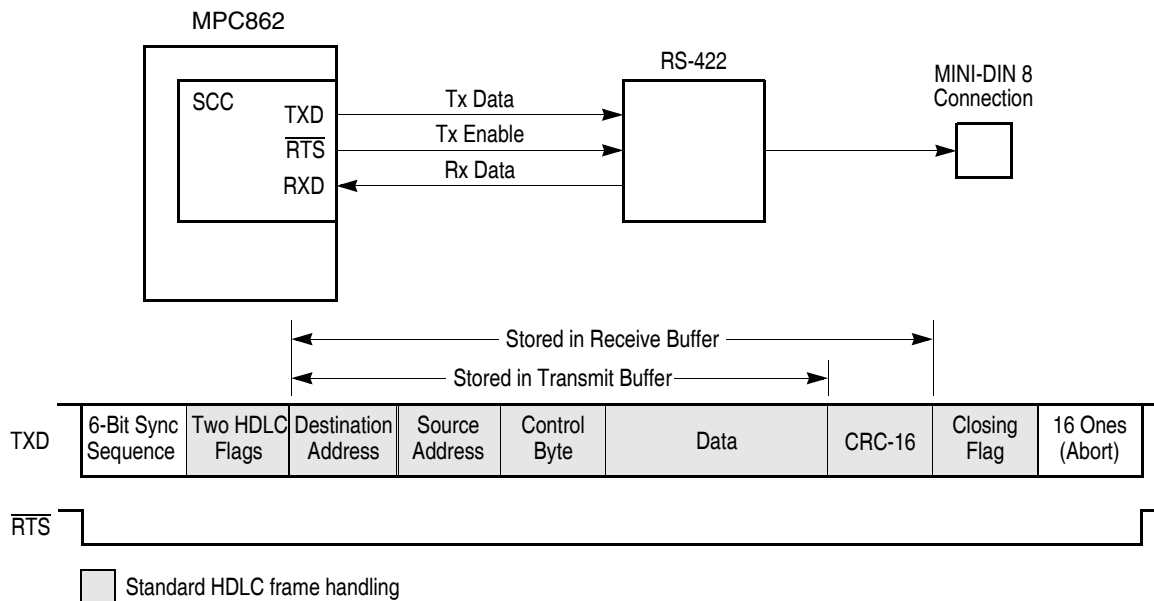
Figure 24-2. Connecting the MPC862 to LocalTalk
