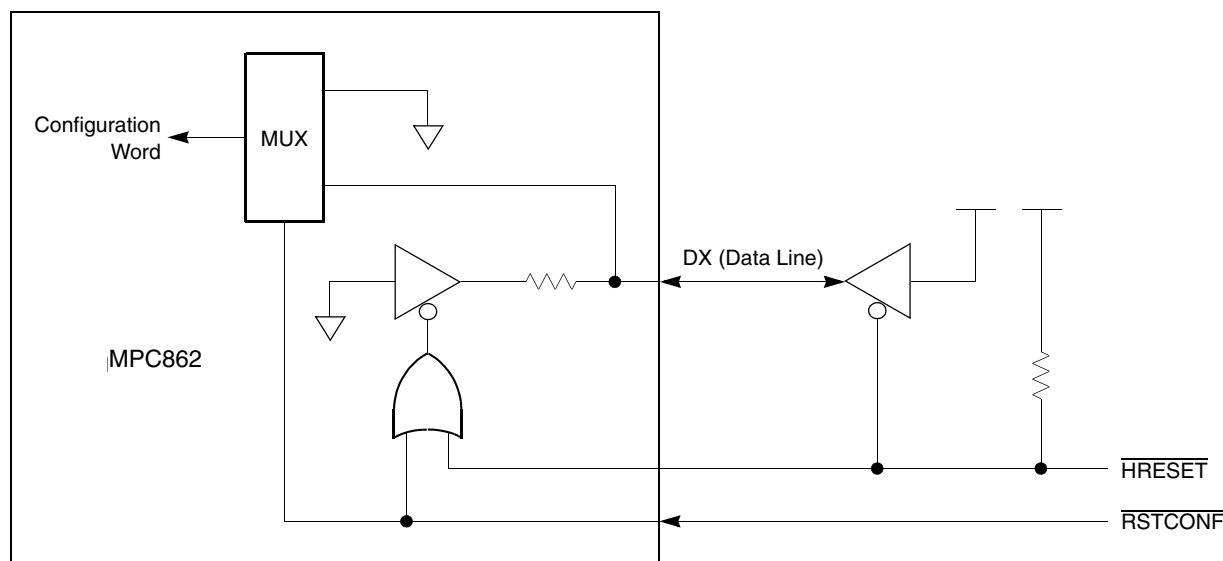
Figure 11-4. Data Bus Configuration Input Circuit
