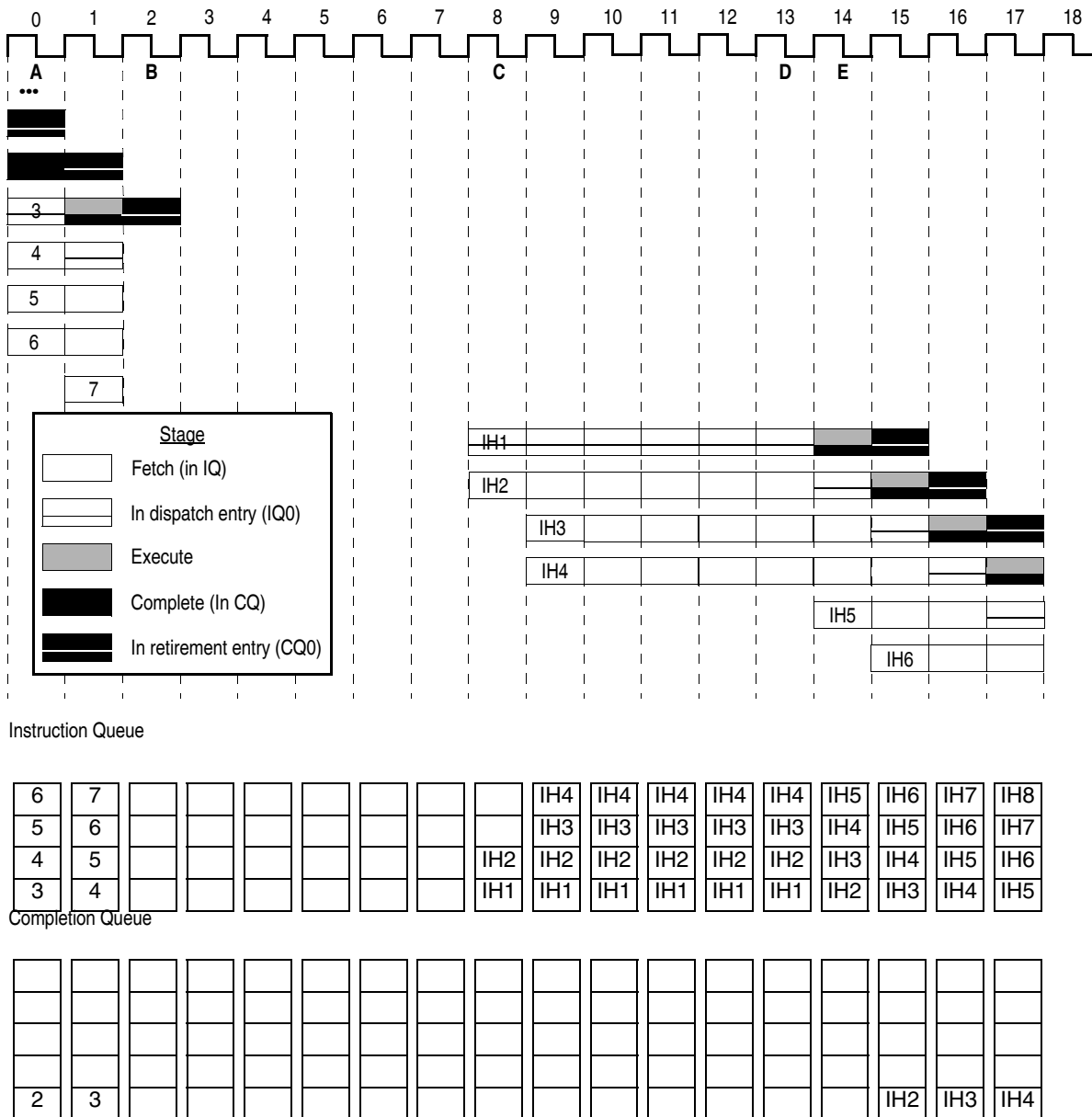
Figure 6-1. Exception Latency
