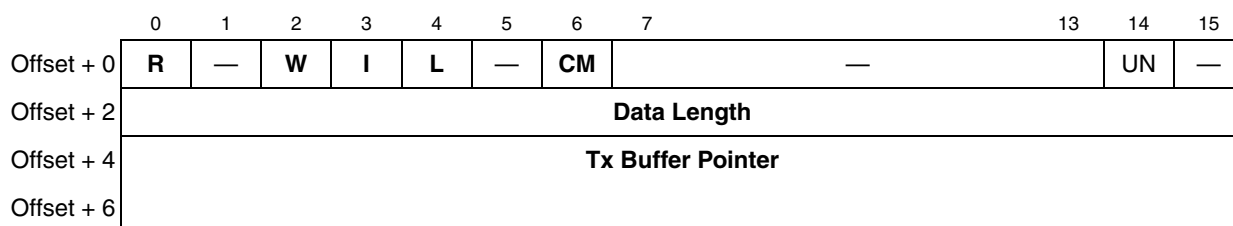
Figure 29-14. SMC Transparent Transmit BD (TxBD)
