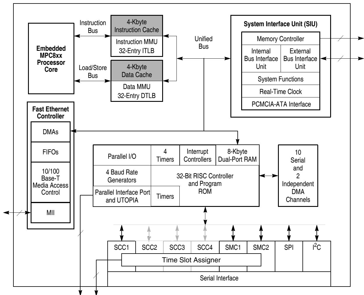
Figure F-1. MPC857T Block Diagram
