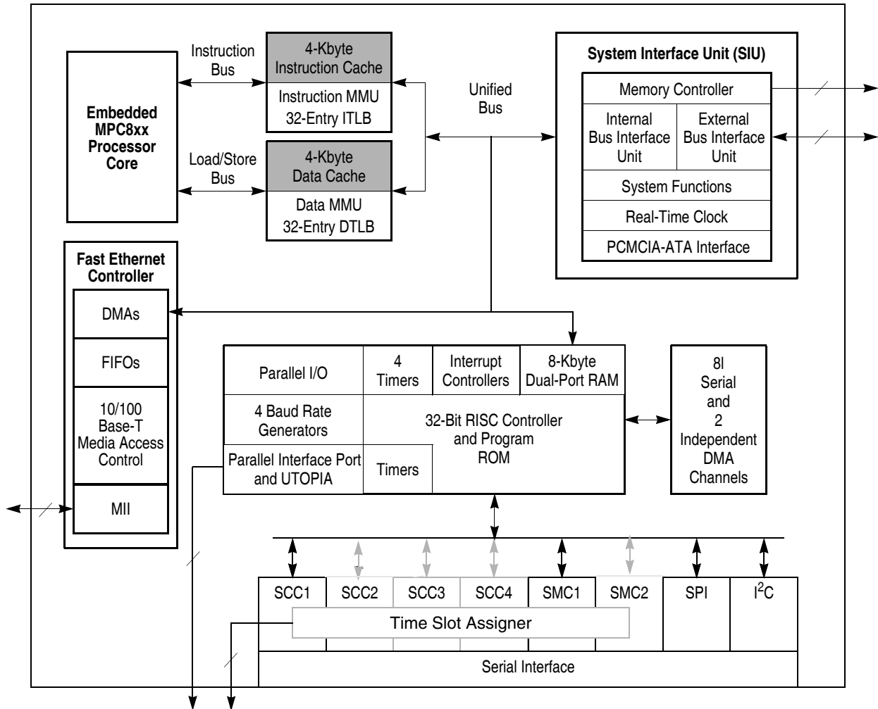
Figure G-1. MPC857DSL Block Diagram
