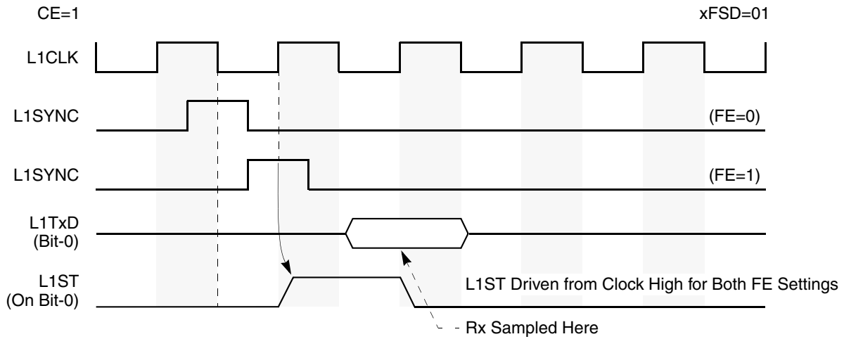
Figure 20-16. Falling Edge (FE) Affect When CE = 1 and xFSD = 01
