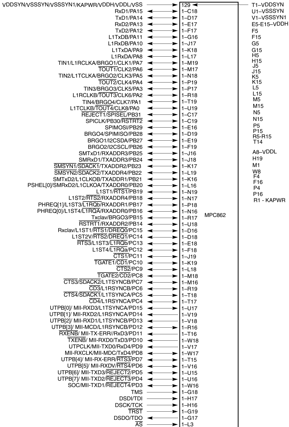
Figure 12-2. Signals and Pin Numbers (Part 1)
