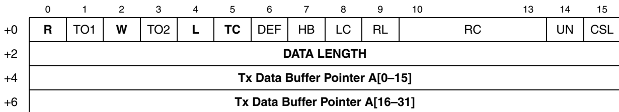
Figure 44-27. Transmit Buffer Descriptor (TxBD)
