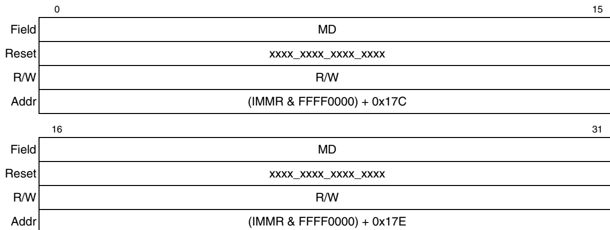
Figure 15-12. Memory Data Register (MDR)
