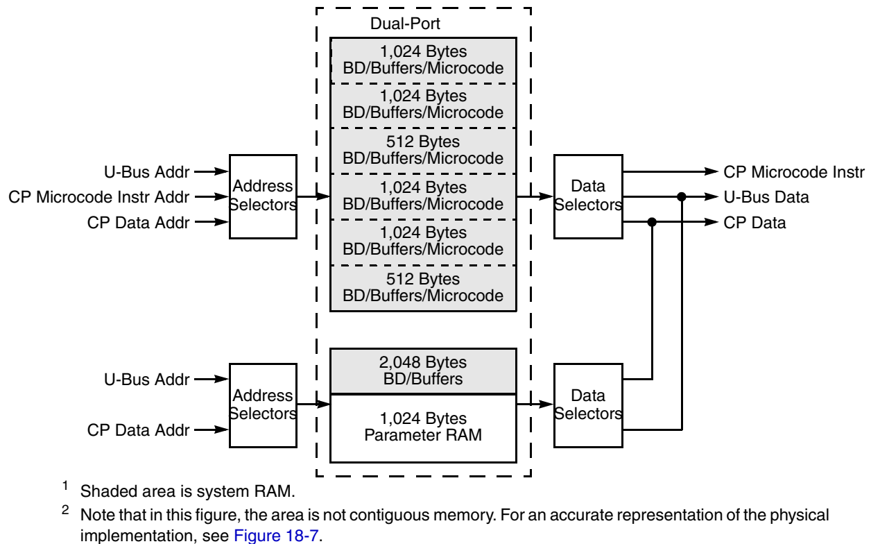
Figure 18-6. Dual-Port RAM Block Diagram
