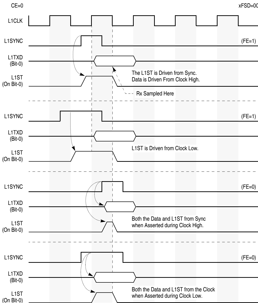
Figure 20-19. Falling Edge (FE) Affect When CE = 0 and xFSD = 00
