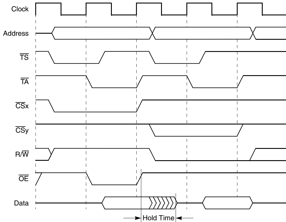
Figure 15-25. GPCM Read Followed by Write ( \overline{EHTR} = 0 )
