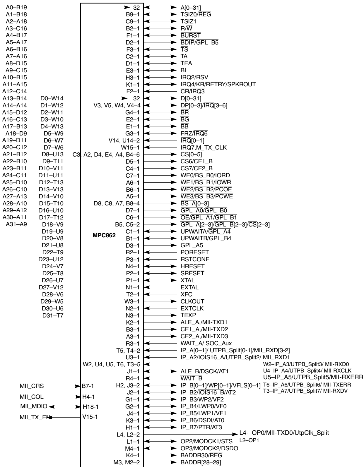
Figure 12-3. Signals and Pin Numbers (Part 2)
