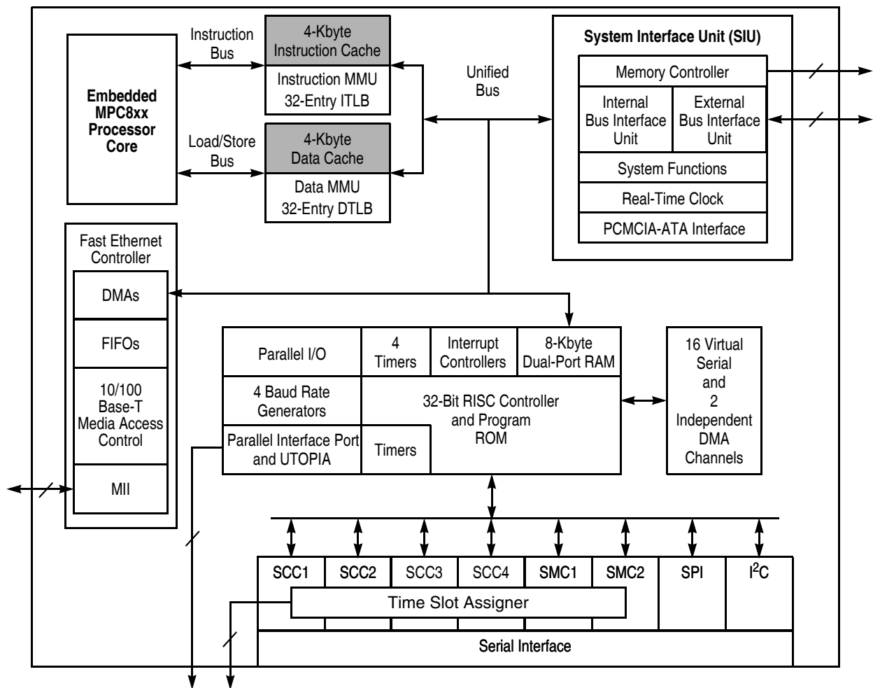
Figure E-1. MPC862T Block Diagram
