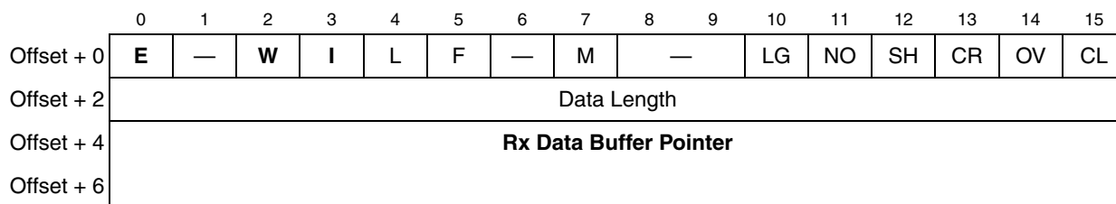
Figure 27-8. SCC Ethernet RxBD
