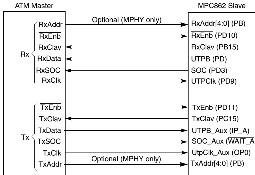
Figure 42-2. UTOPIA Slave Interface with Split Bus
