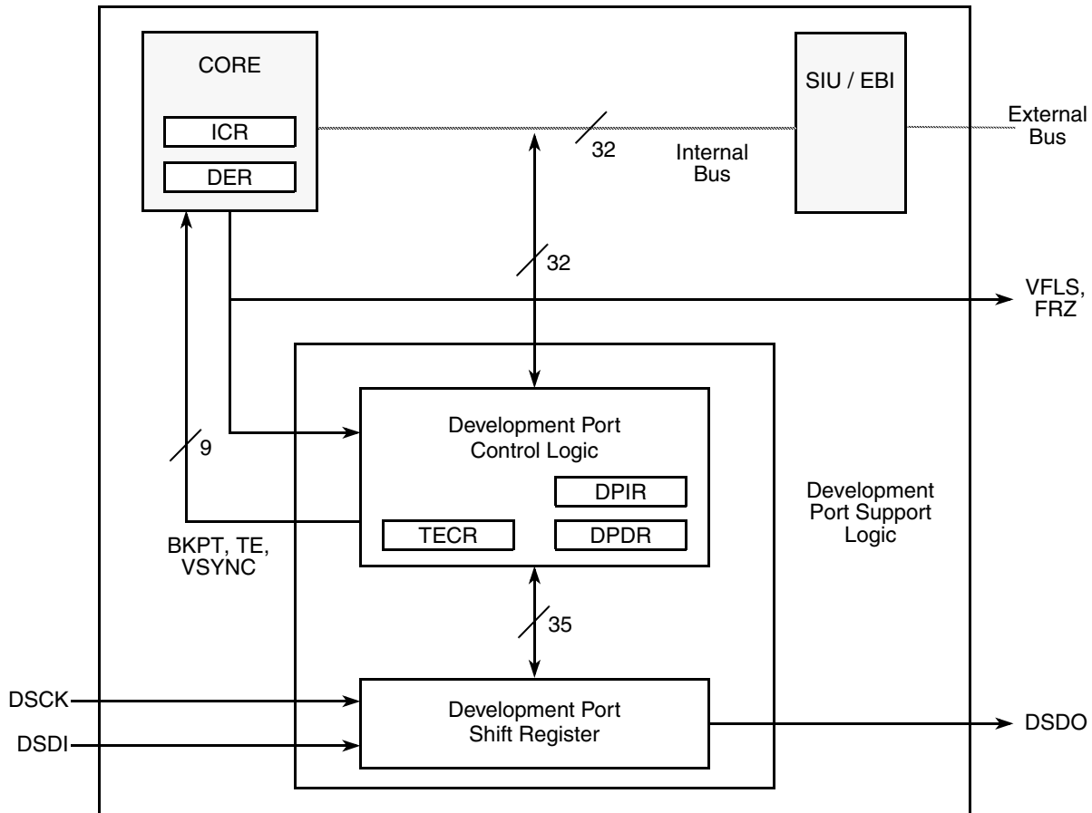
Figure 45-5. Functional Diagram of the MPC862 Debug Mode Support
