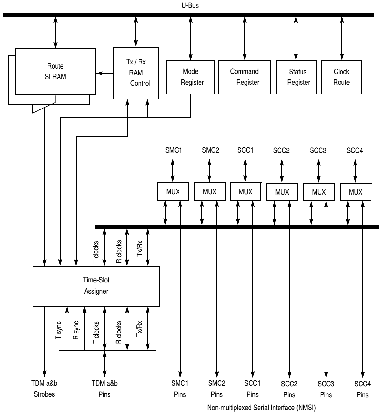
Figure 20-1. MPC862 SI Block Diagram
