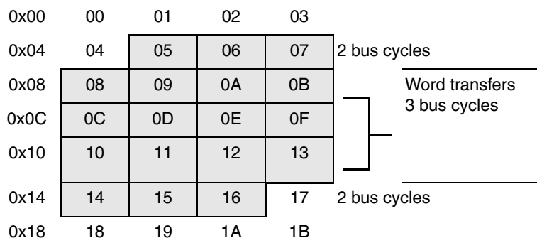
Figure 9-9. Bus Latency for String Instructions
