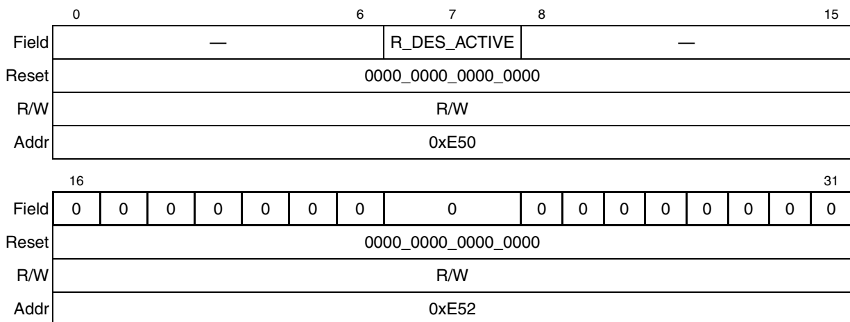
Figure 44-14. R_DES_ACTIVE Register
