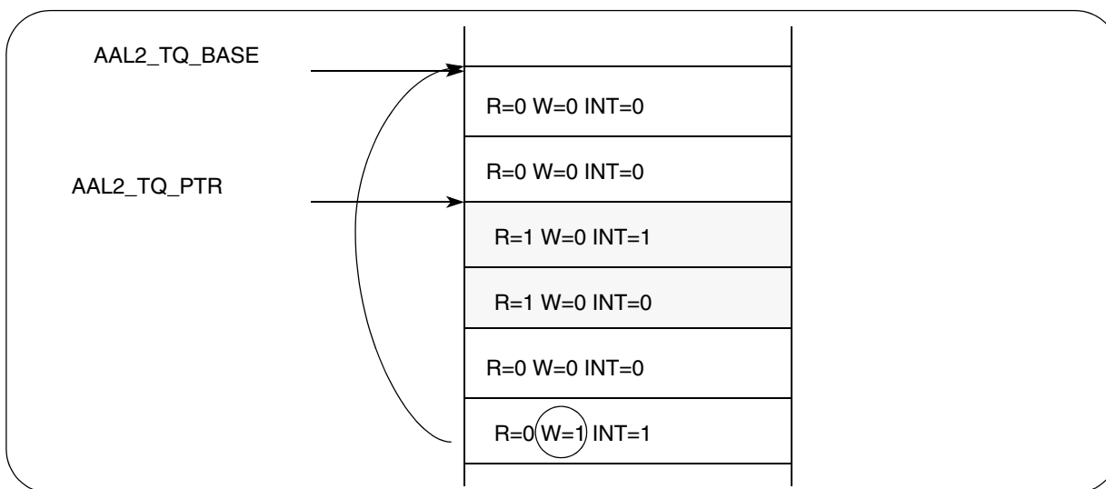
Figure 43-2. AAL2_Tx_Queue Example
