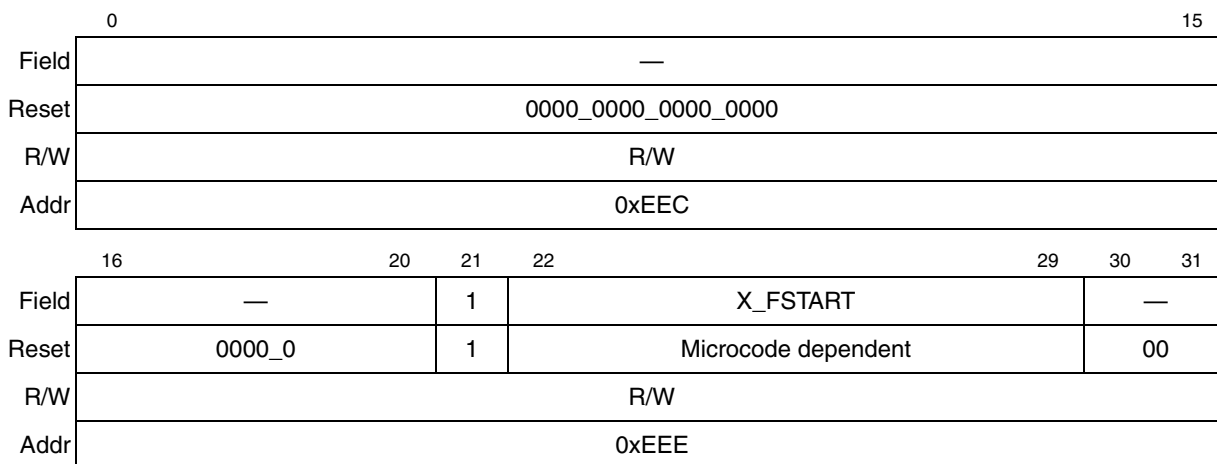
Figure 44-21. X_FSTART Register
