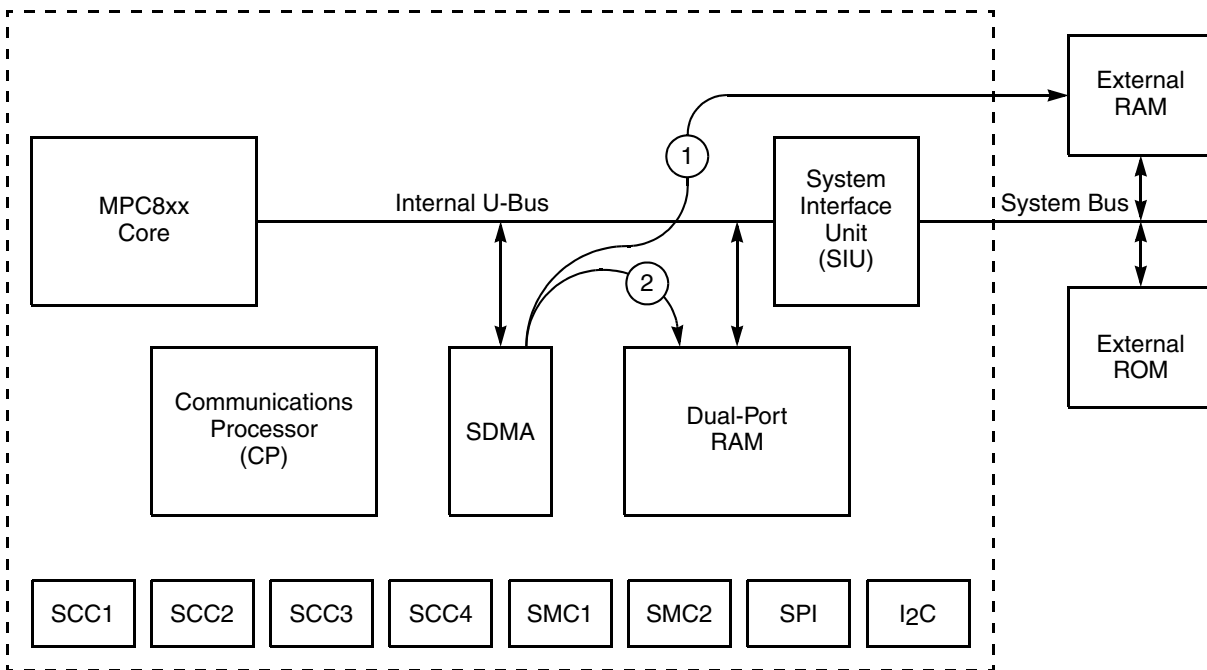
Figure 19-1. MPC862 SDMA Data Paths
