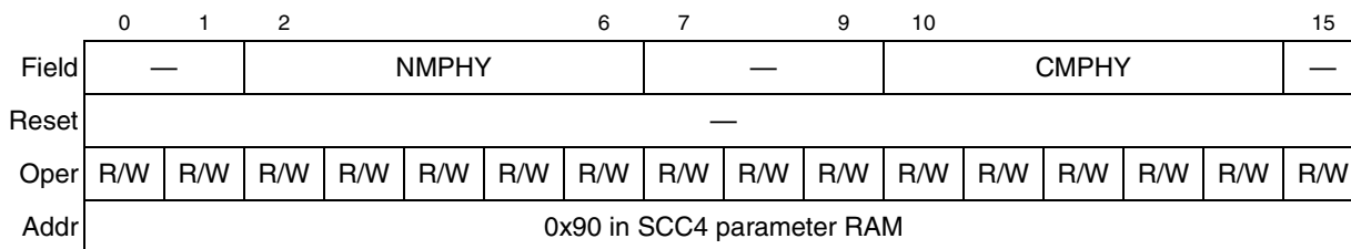
Figure 37-8. MPHY State Register (MPHYST)
