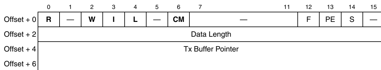
Figure 32-9. PIP Tx Buffer Descriptor (TxBD)
