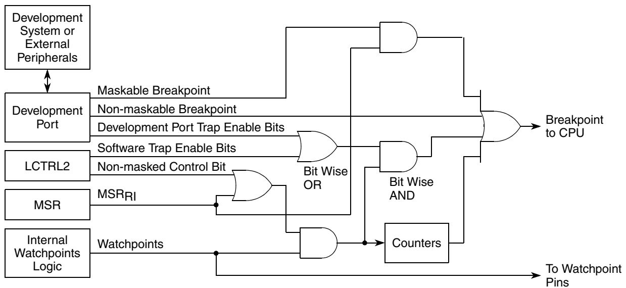
Figure 45-1. Watchpoints and Breakpoint Support in the Core
