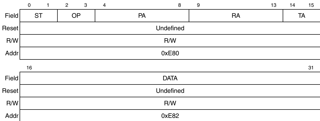
Figure 44-16. MII_DATA Register
