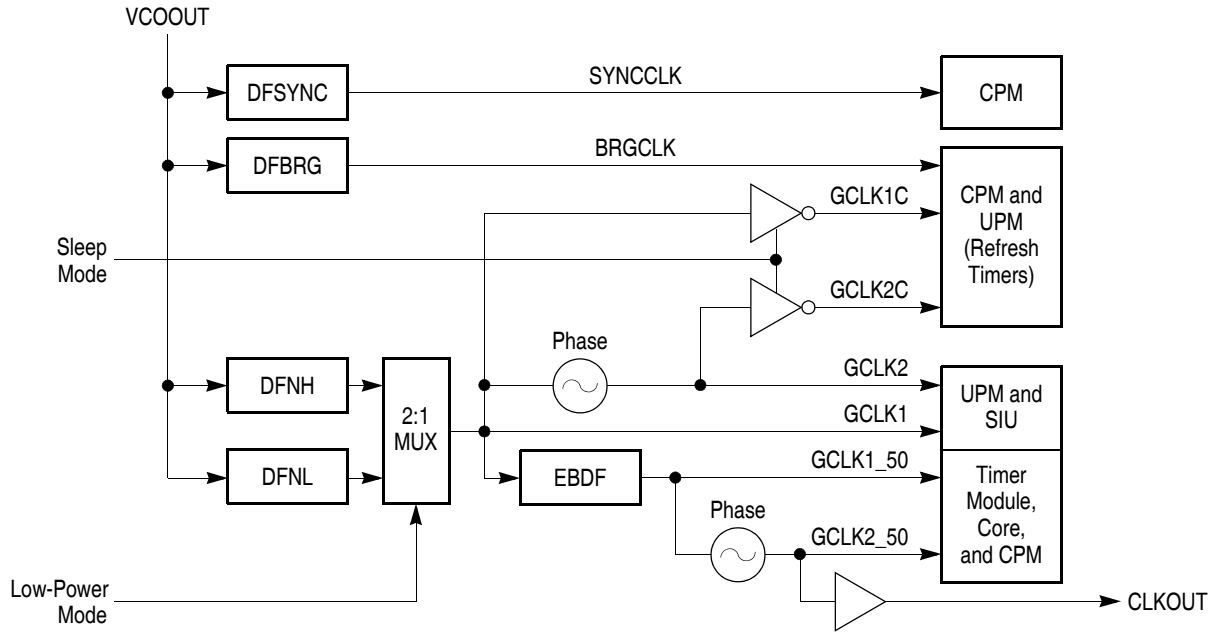
Figure 14-5. Clock Dividers
