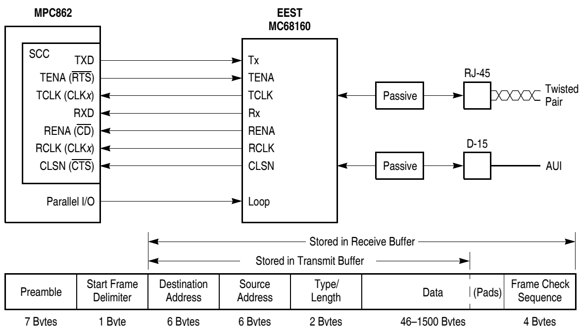
Figure 27-3. Connecting the MPC862 to Ethernet
