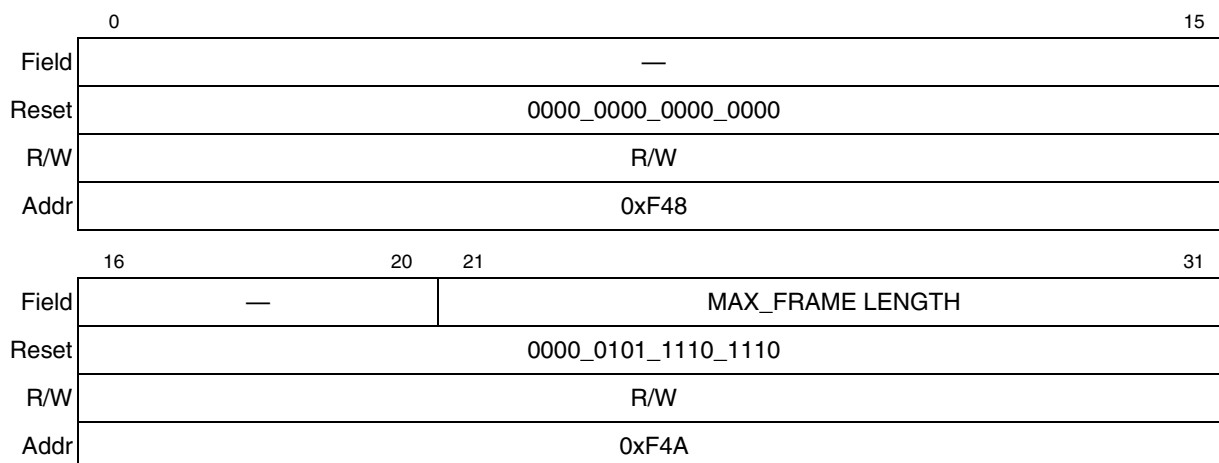
Figure 44-24. R_HASH Register
