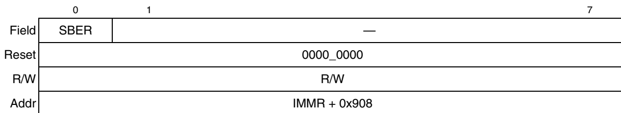
Figure 19-4. SDMA Status Register (SDSR)
