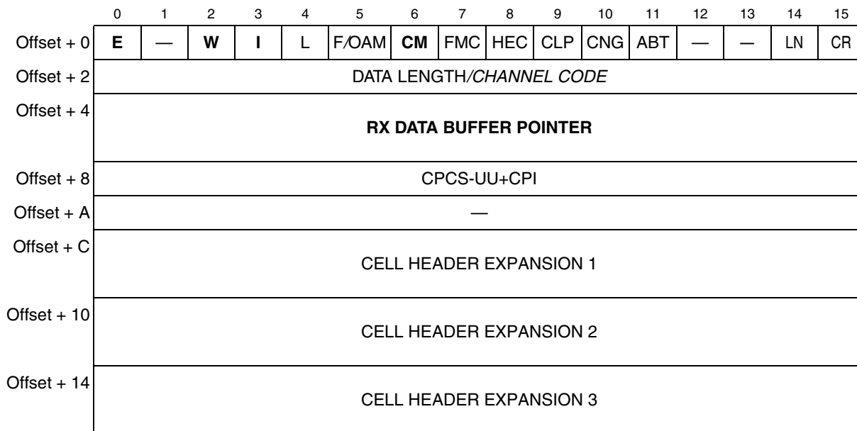
Figure 36-4. ATM RxBD in Expanded Cell Mode (UTOPIA Only)
