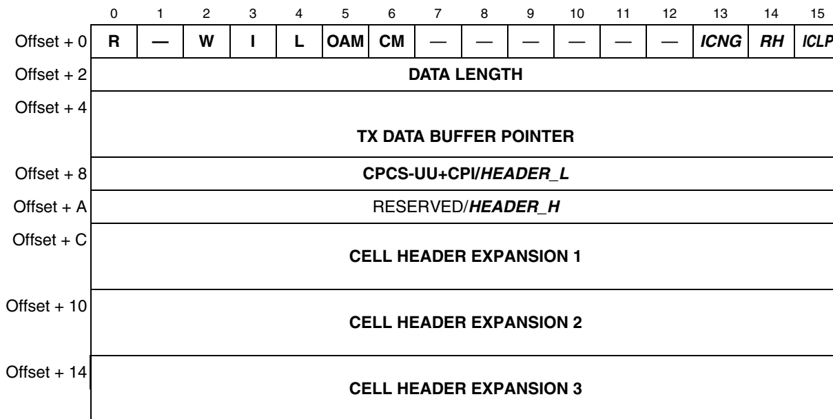
Figure 36-6. ATM TxBD in Expanded Cell Mode (UTOPIA Only)
