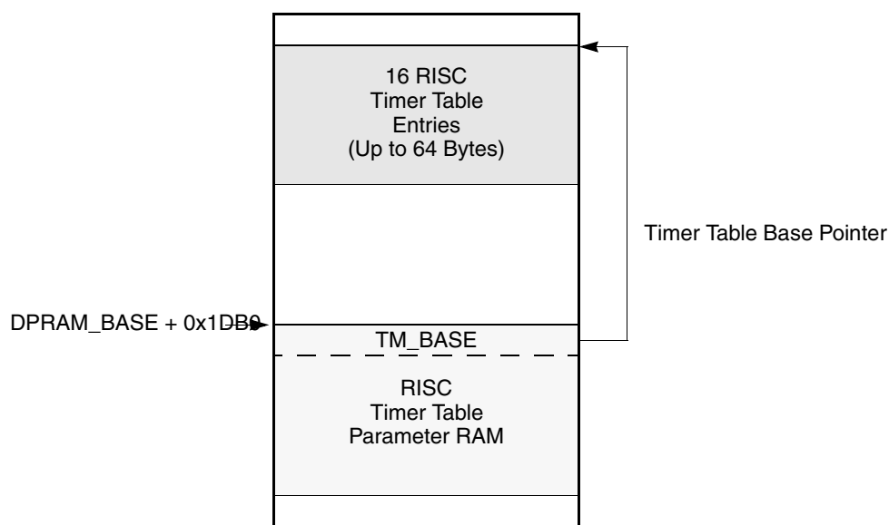
Figure 18-8. RISC Timer Table RAM Usage
