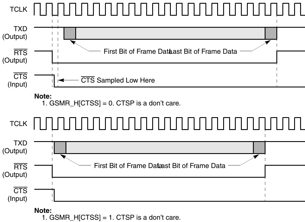
Figure 21-10. Output Delay from \overline{\text{CTS}} Asserted for Synchronous Protocols
