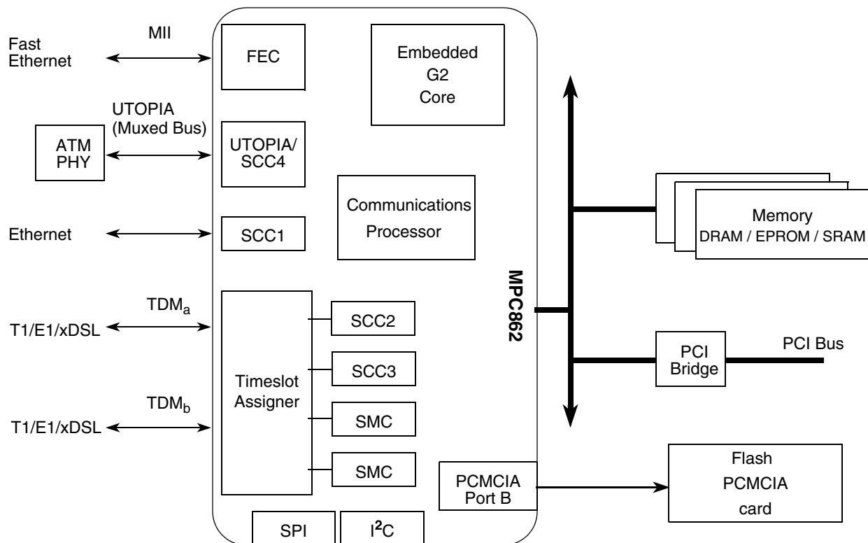
Figure 35-2. MPC862 Application Example
