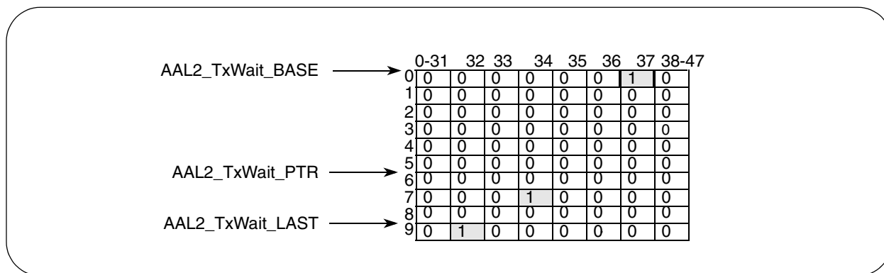
Figure 43-5. Example of the Wait Table
