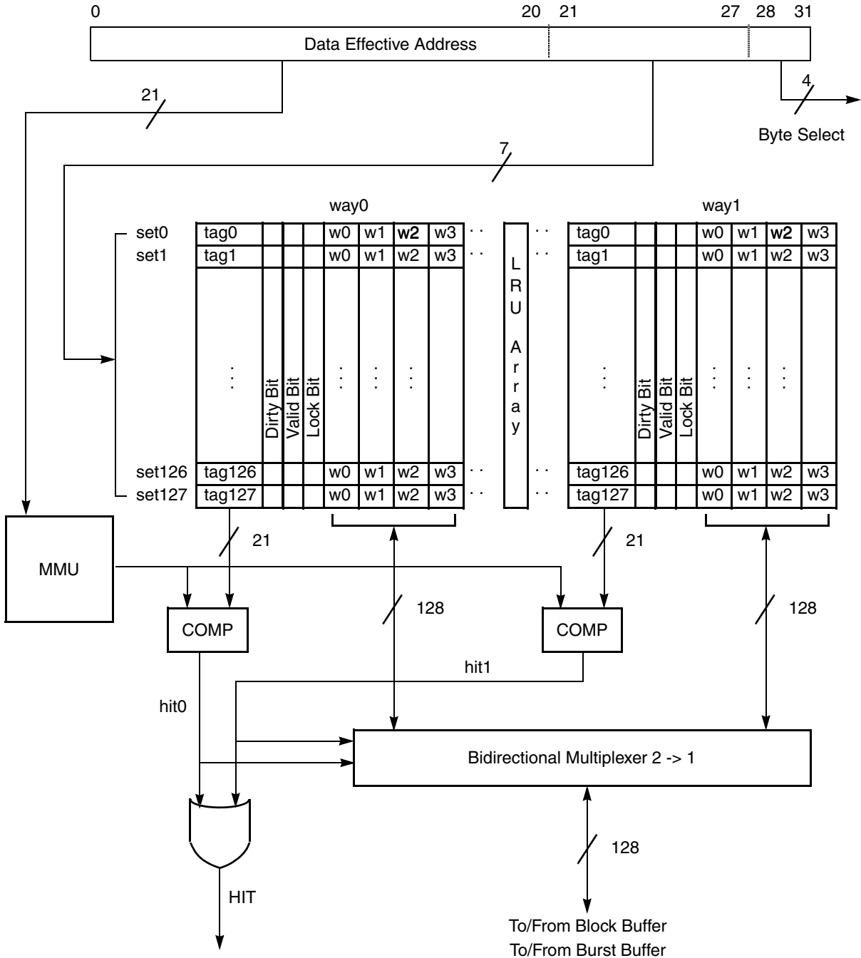
Figure 7-4. MPC862T/MPC857T/MPC857DSL Data Cache Organization
