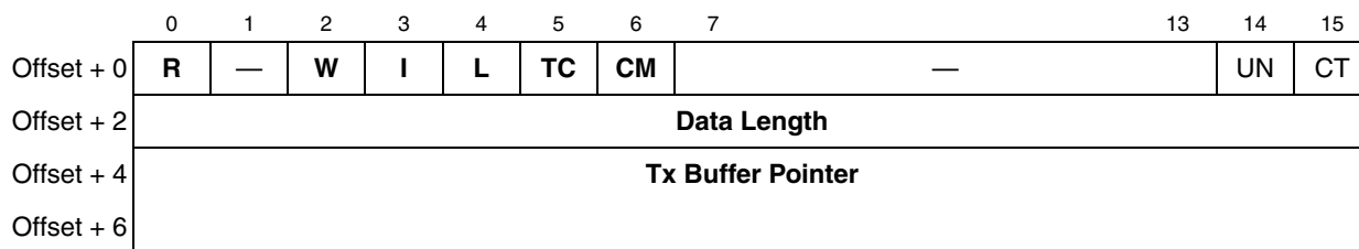
Figure 23-6. SCC HDLC Transmit Buffer Descriptor (TxBD)
