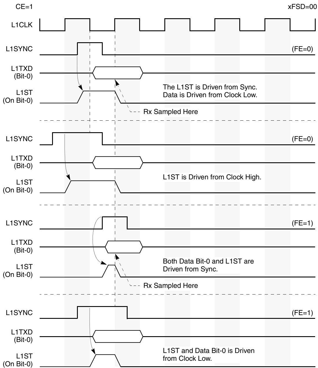
Figure 20-18. Falling Edge (FE) Affect When CE = 1 and xFSD = 00
