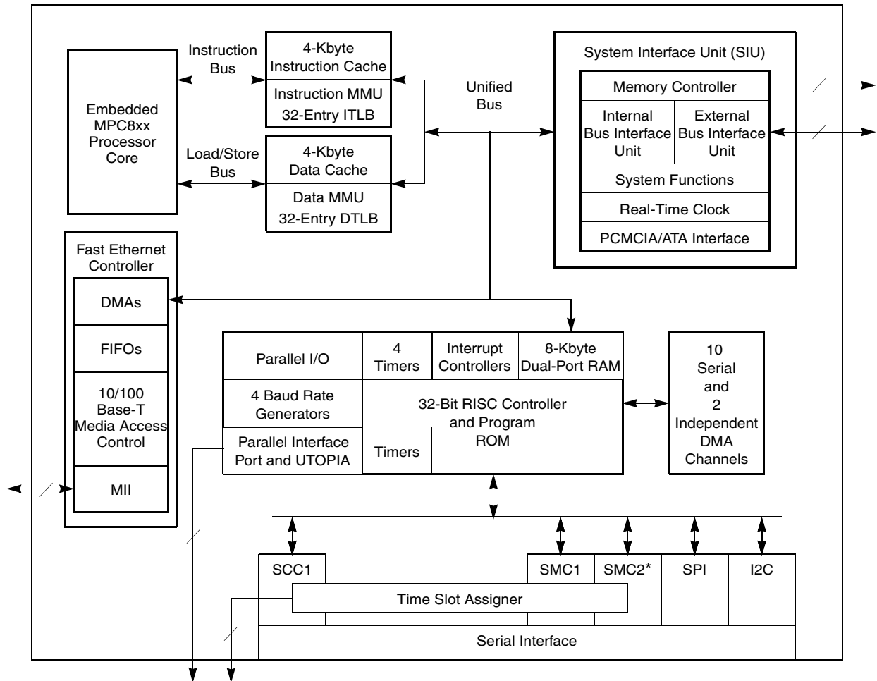
Figure 1-2. MPC857T/MPC857DSL Block Diagram
