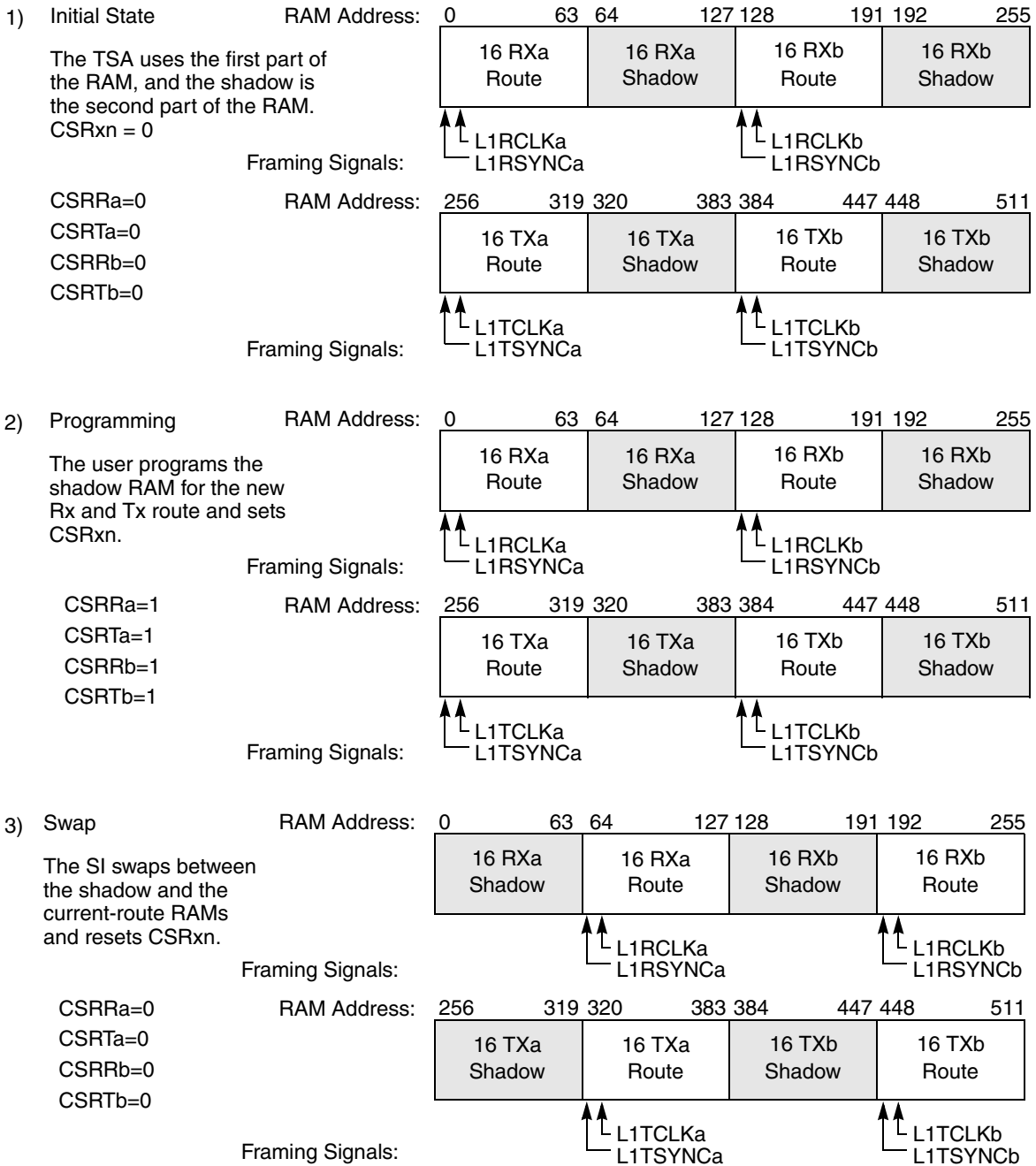
Figure 20-7. SI RAM Dynamic Changes with TDMA and TDMb
