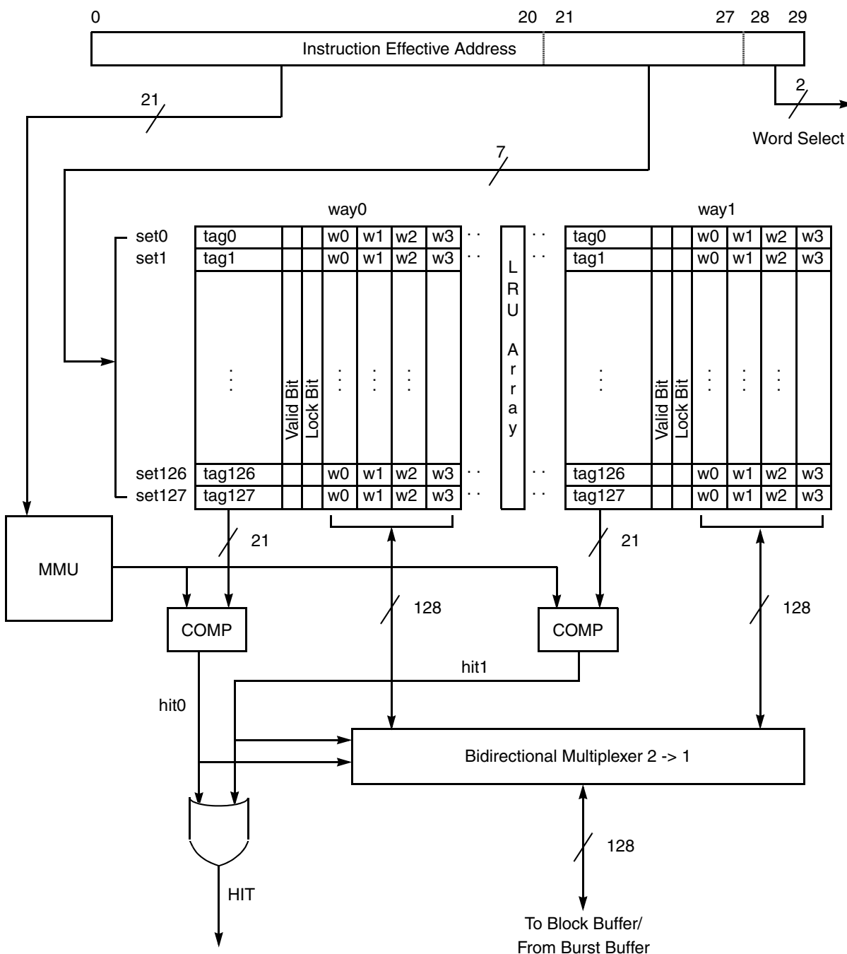
Figure 7-2 shows the organization of the 4-Kbyte MPC862T/MPC857T/MPC857DSL instruction cache.
