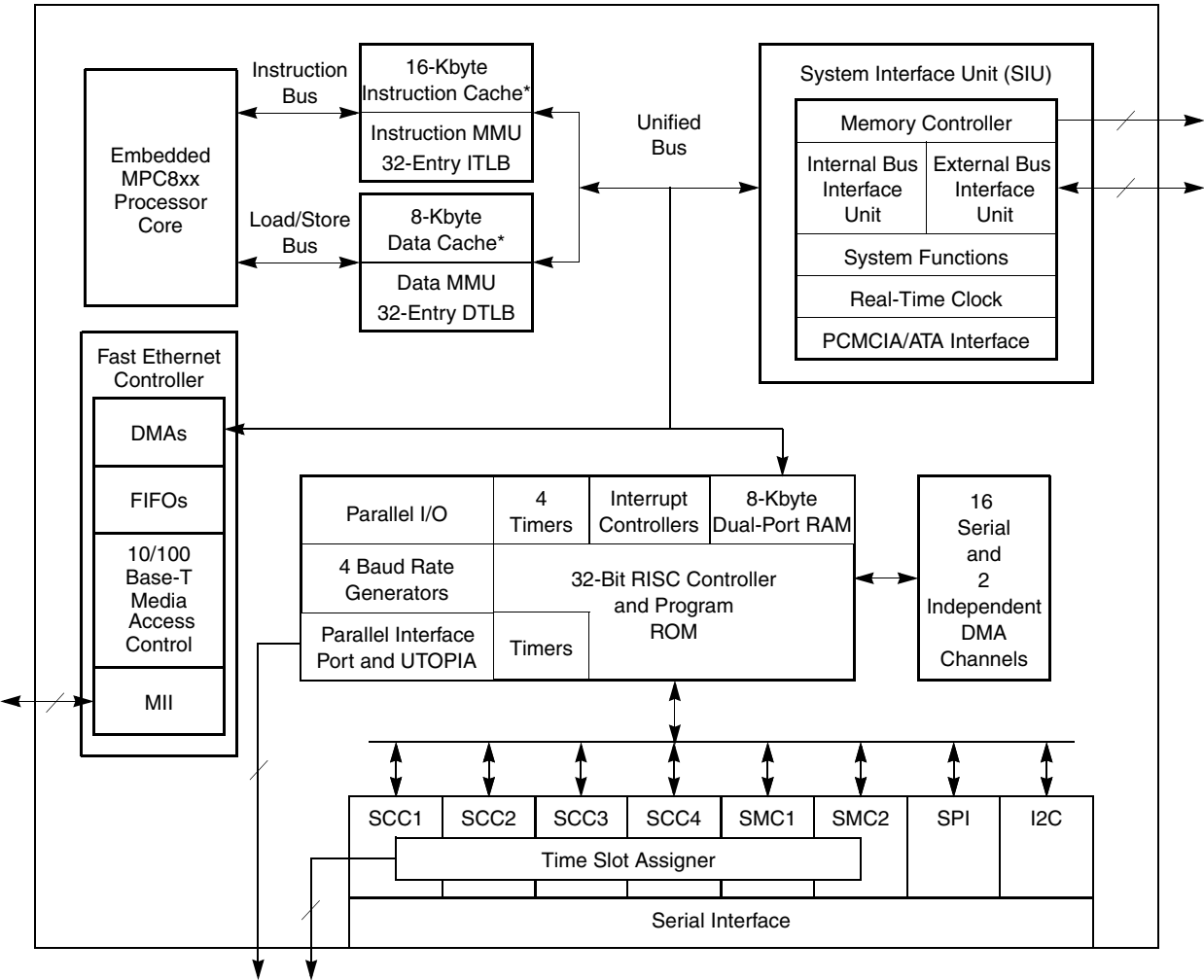
Figure 1-1. MPC862P/862T Block Diagram
