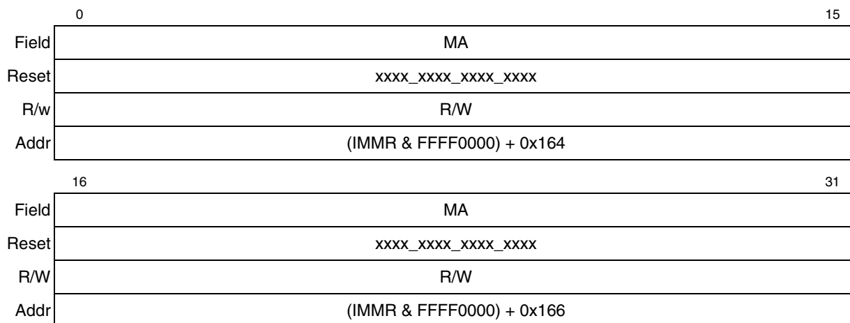
Figure 15-13. Memory Address Register (MAR)
