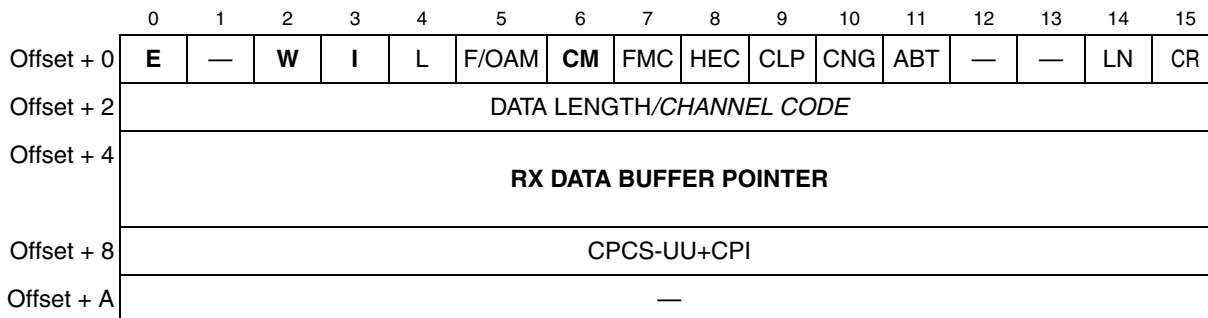
Figure 36-3. ATM RxBd
