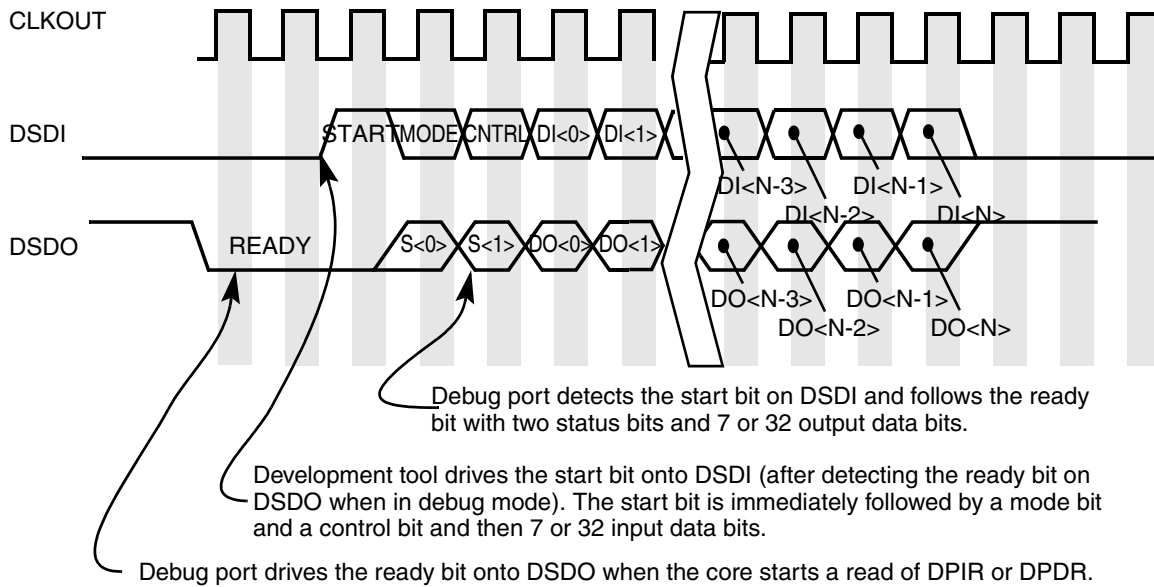
Figure 45-10. Synchronous Self-Clocked Serial Communications
