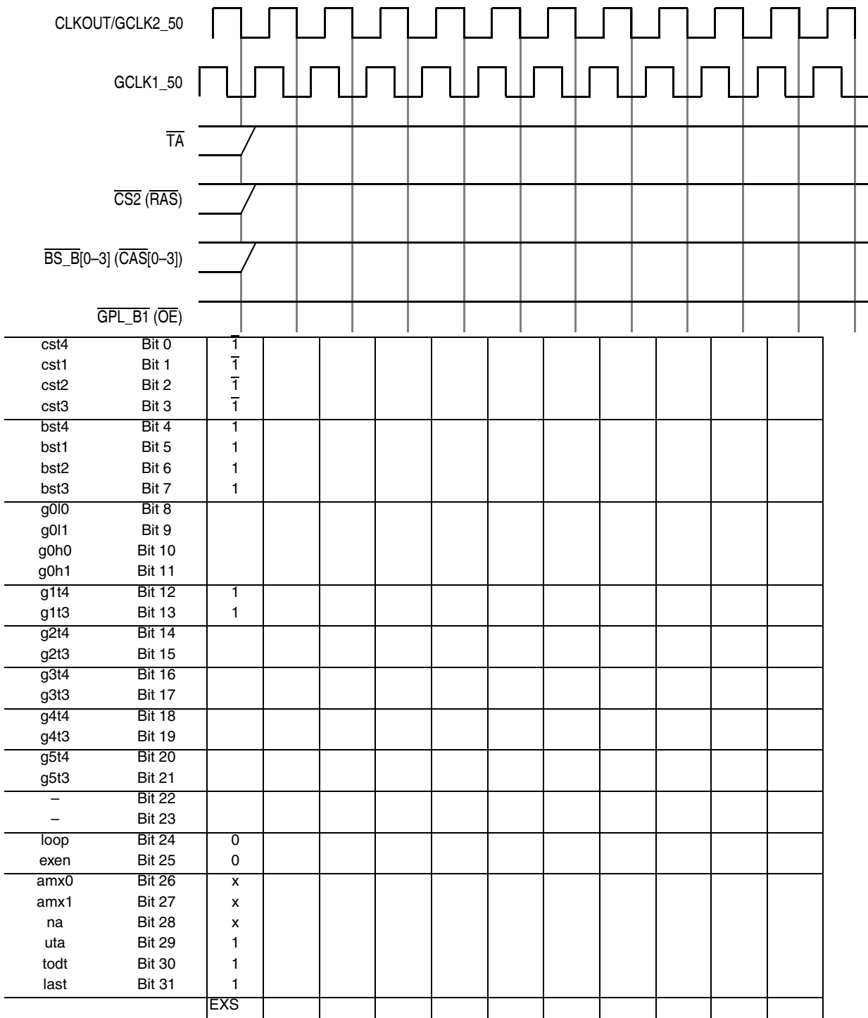
Figure 15-69. EDO DRAM Exception Cycle
