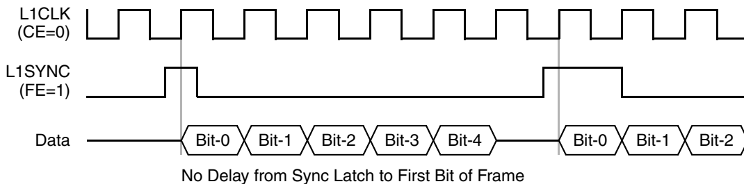
Figure 20-15. No Delay from Sync to Data (xFS D = 00)
