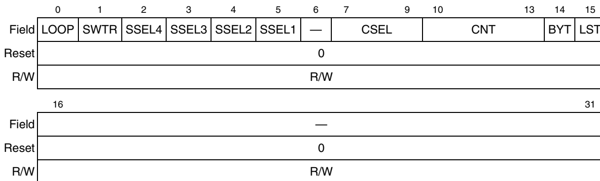
Figure 20-10. S1RAM Entry
