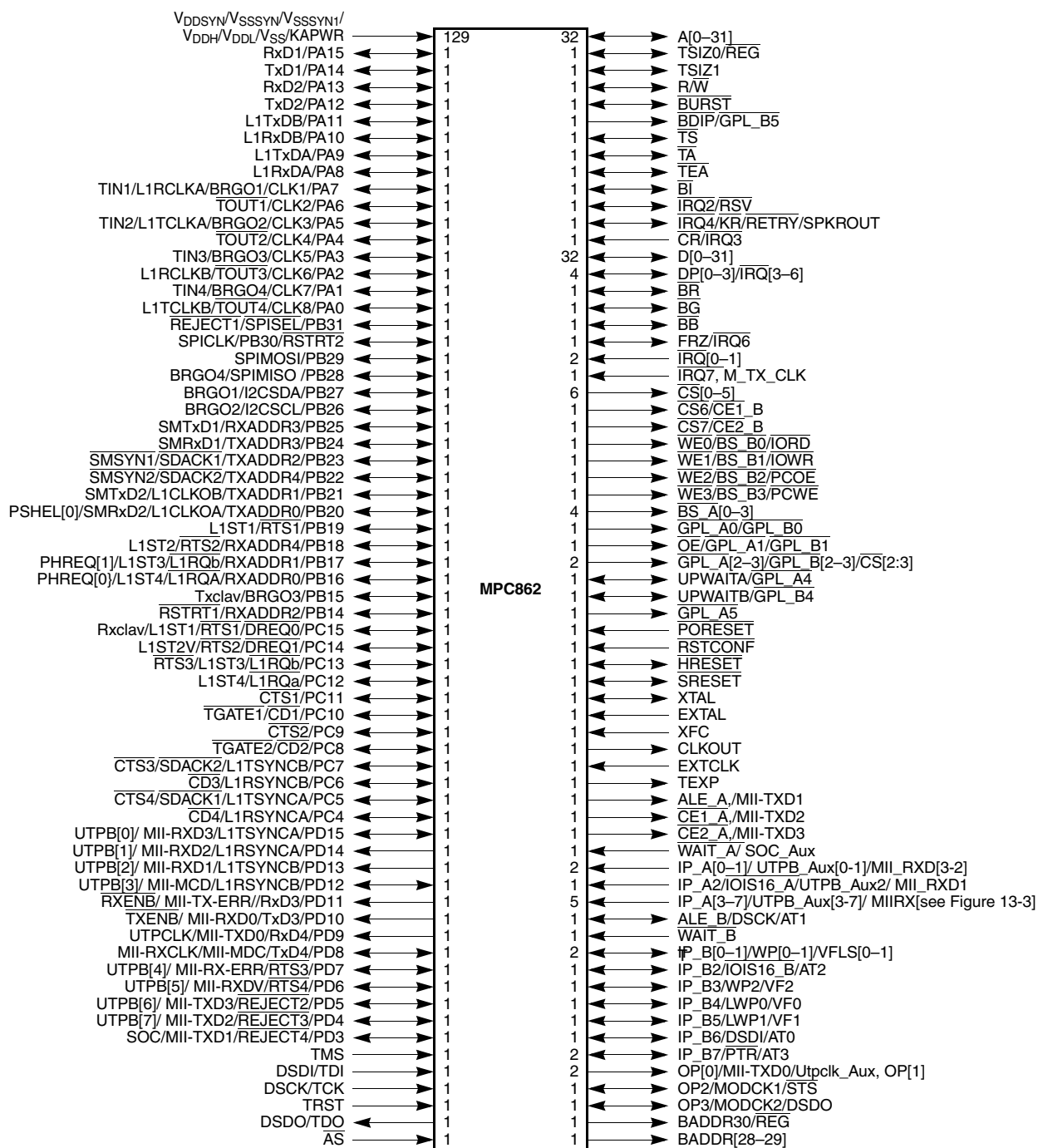
Figure 12-1. MPC862 External Signals
