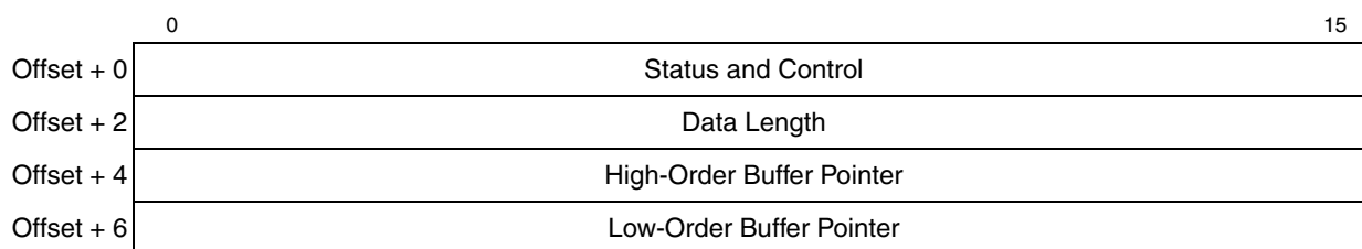
Figure 21-6. SCC Buffer Descriptors (BDs)
