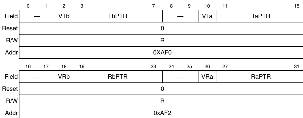
Figure 20-23. SI RAM Pointer Register (SIRP)
