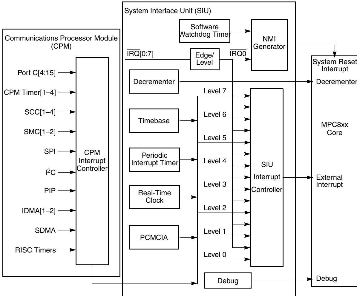
Figure 34-1. MPC862 Interrupt Structure
