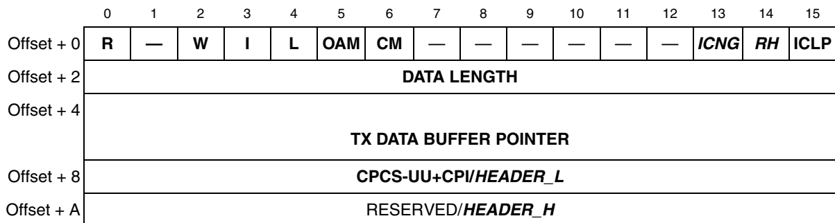
Figure 36-5. ATM TxBD
