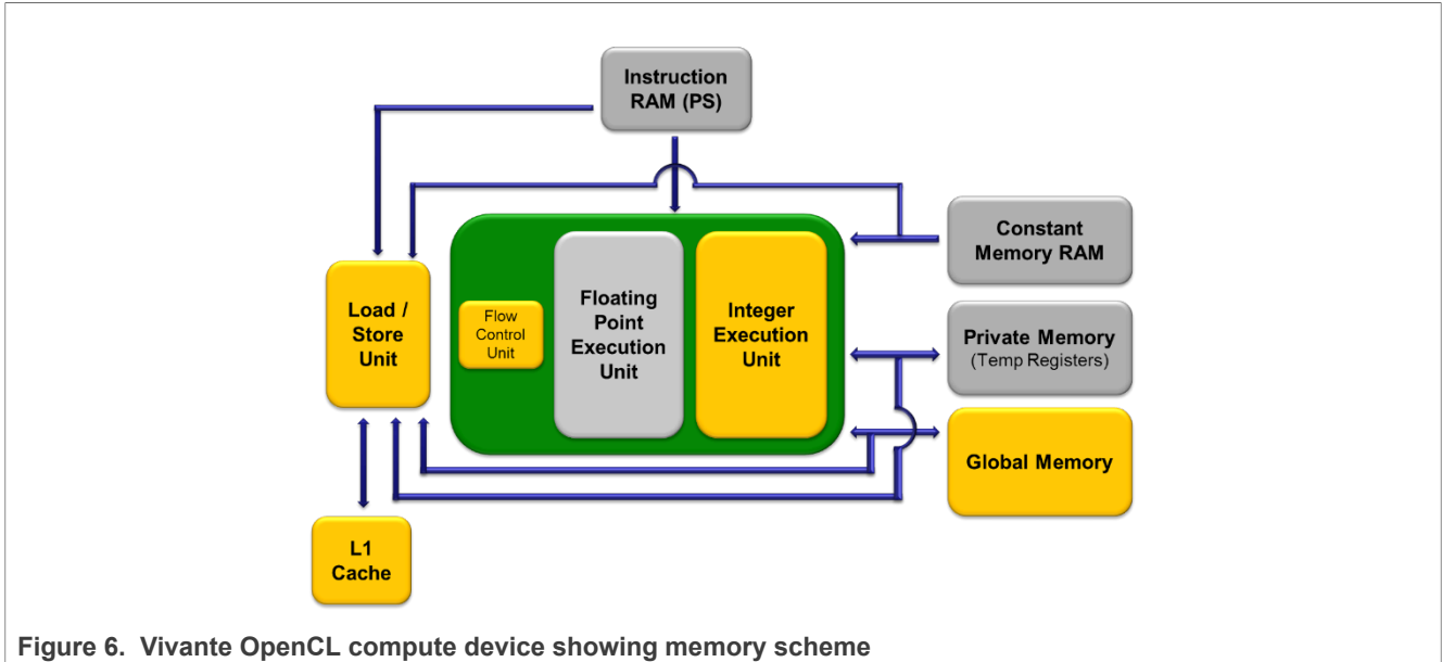
Figure 6. Vivante OpenCL compute device showing memory scheme
