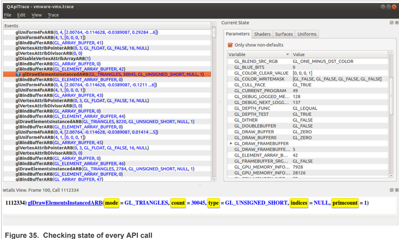
Figure 35. Checking state of every API call
