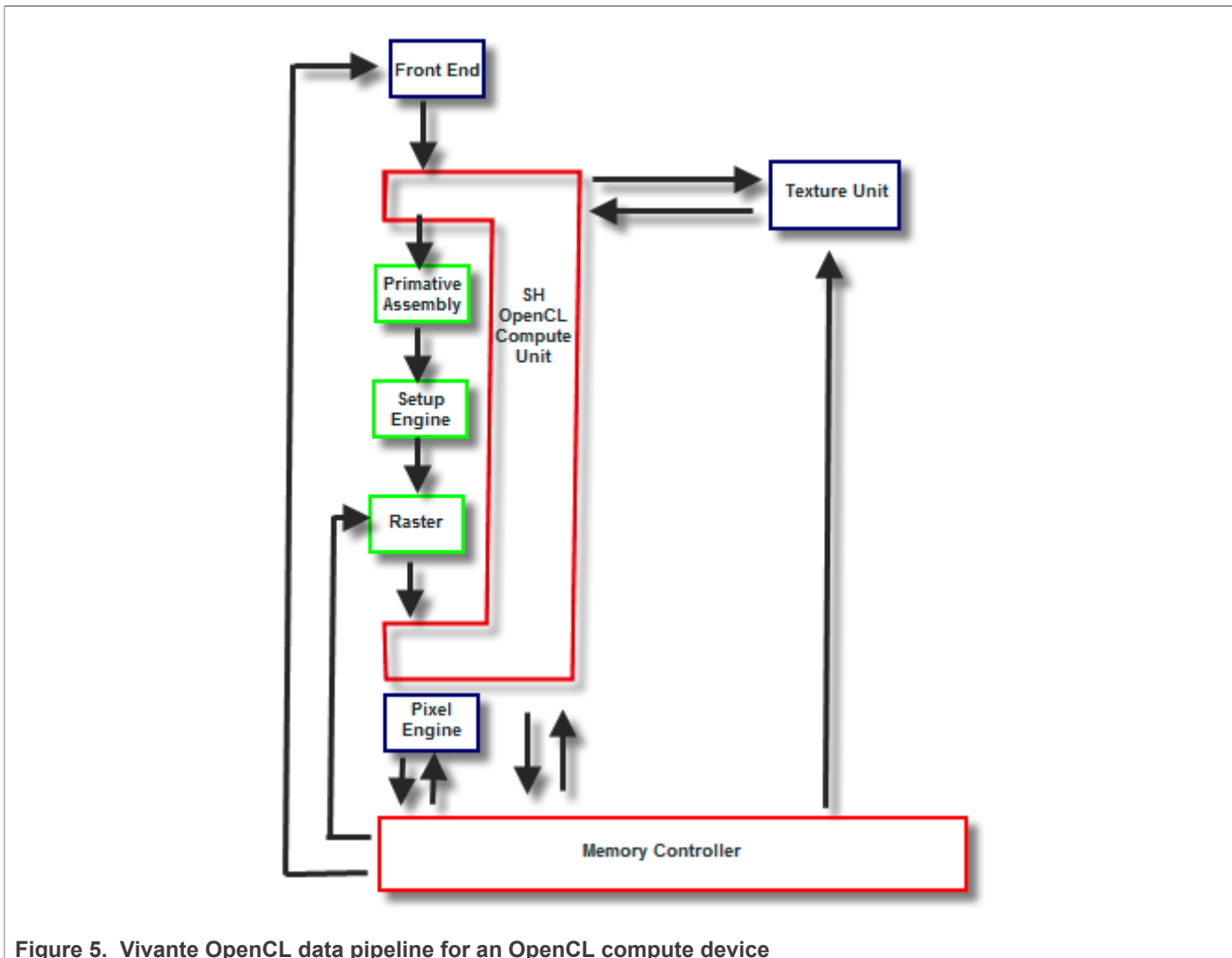
Figure 5. Vivante OpenCL data pipeline for an OpenCL compute device
