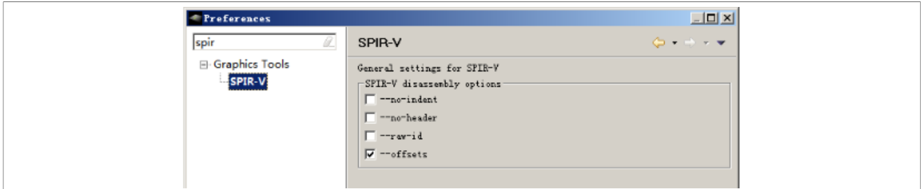
Figure 29. SPIR-V Disassembler
