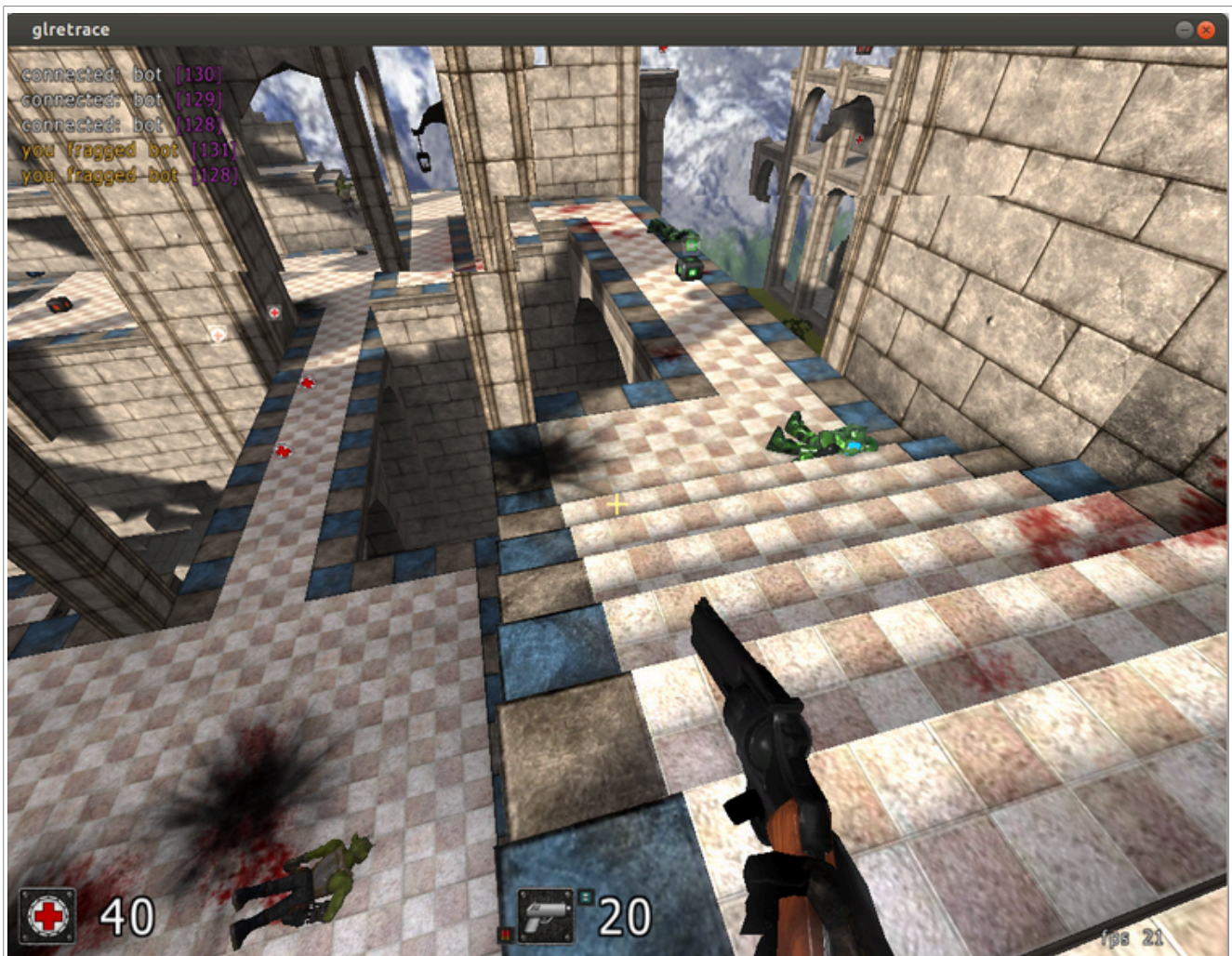
Figure 34. Replay
