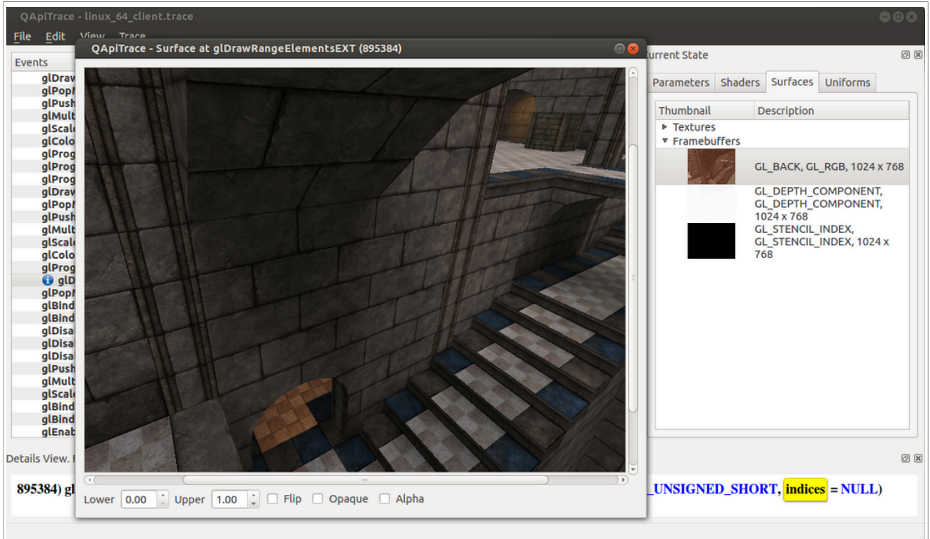
Figure 36. Checking Framebuffer
