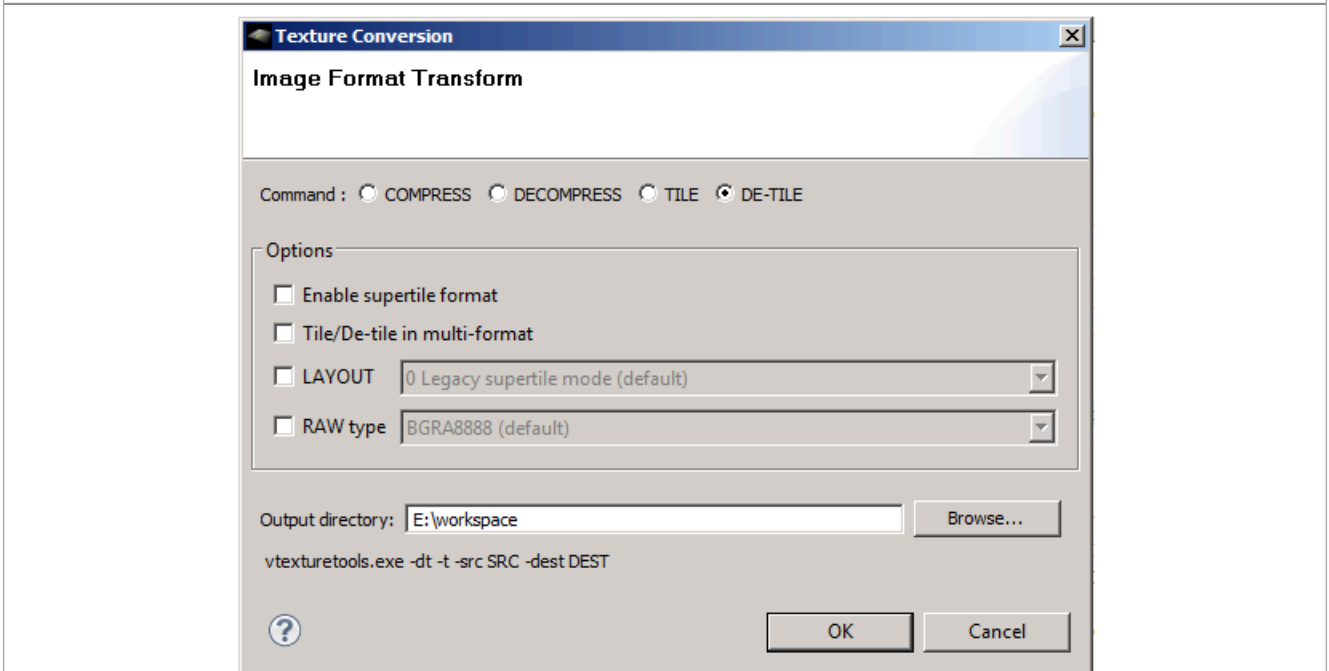
Figure 33. vTexture (3)
