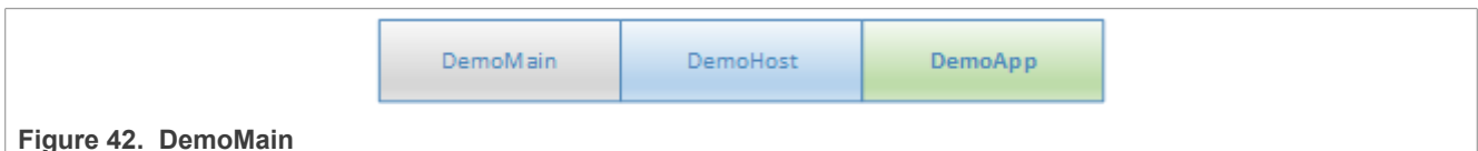
Figure 42. DemoMain
