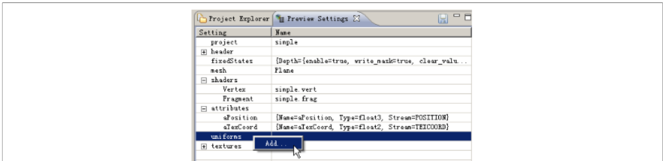
Figure 30. Shader Assistant
