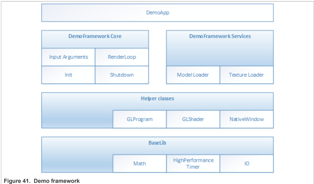
Figure 41. Demo framework
