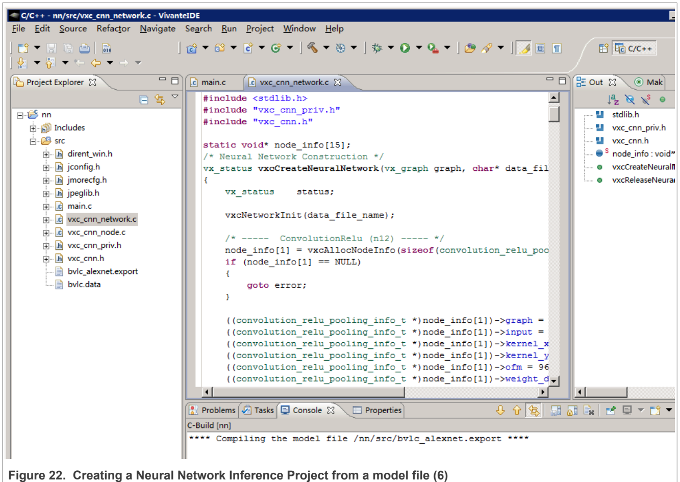
Figure 22. Creating a Neural Network Inference Project from a model file (6)
