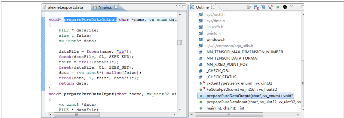
Figure 15. Source code smart editing for OpenVX and OpenCL (1)
