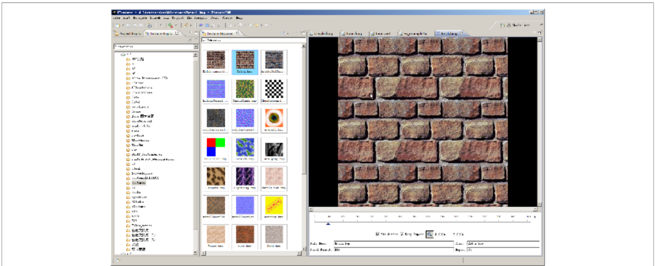
Figure 31. vTexture (1)
