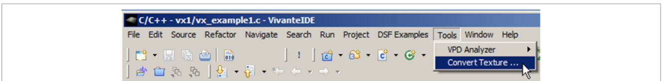
Figure 32. vTexture (2)
