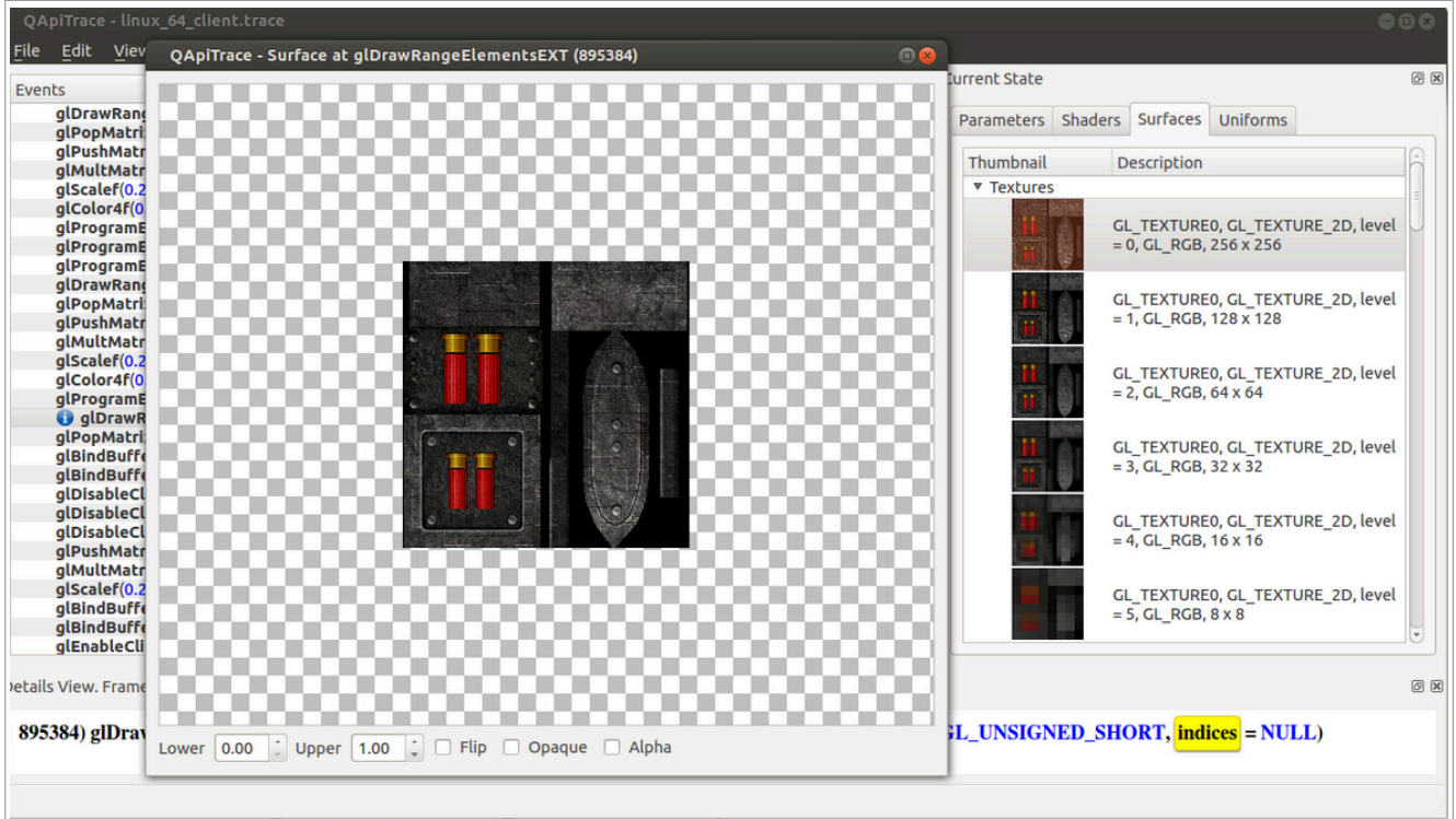
Figure 37. Checking Texture
