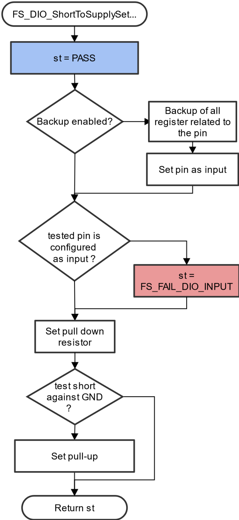
Figure 13. Block diagram of FS_DIO_ShortToSupplySet_IMX8M() function IEC60730_B_CM33_Library_UG_v4_3, Rev. 1, 30. September 2022
