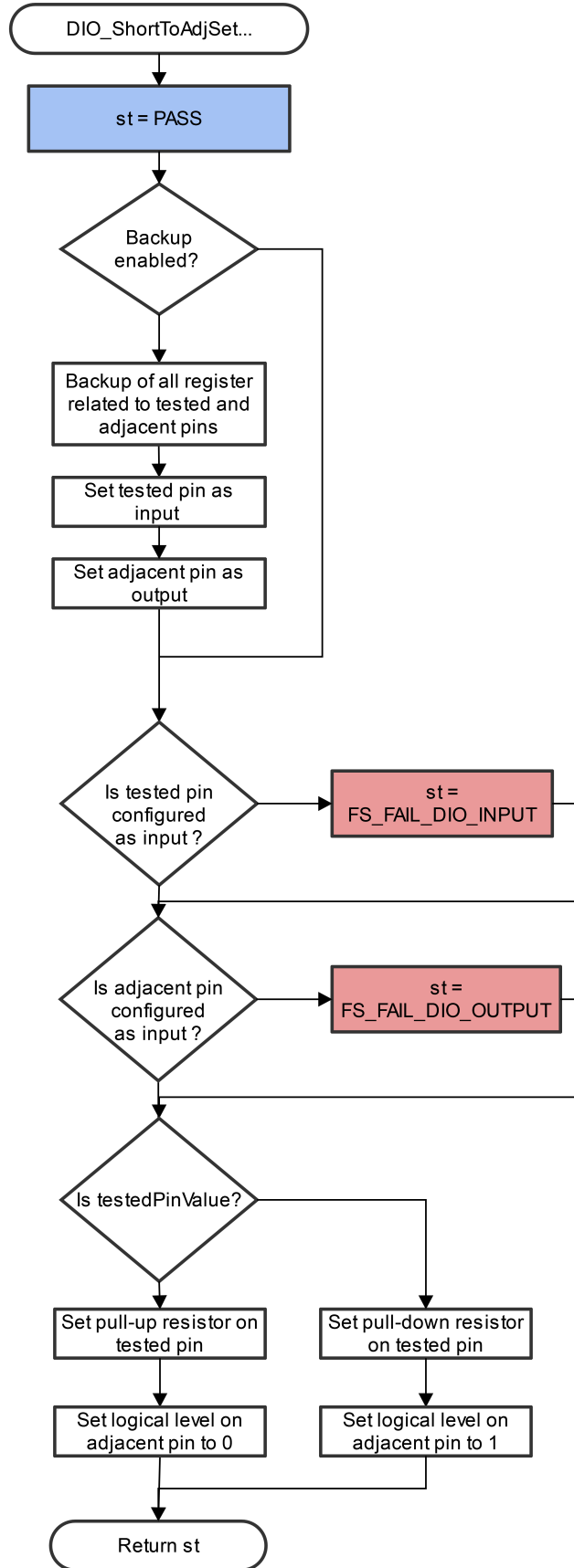
Figure 16. Block diagram of FS_DIO_ShortToAdjSet_IMXRT0 function IEC60730_B_CM33_Library_UG_v4_3, Rev. 1, 30. September 2022
