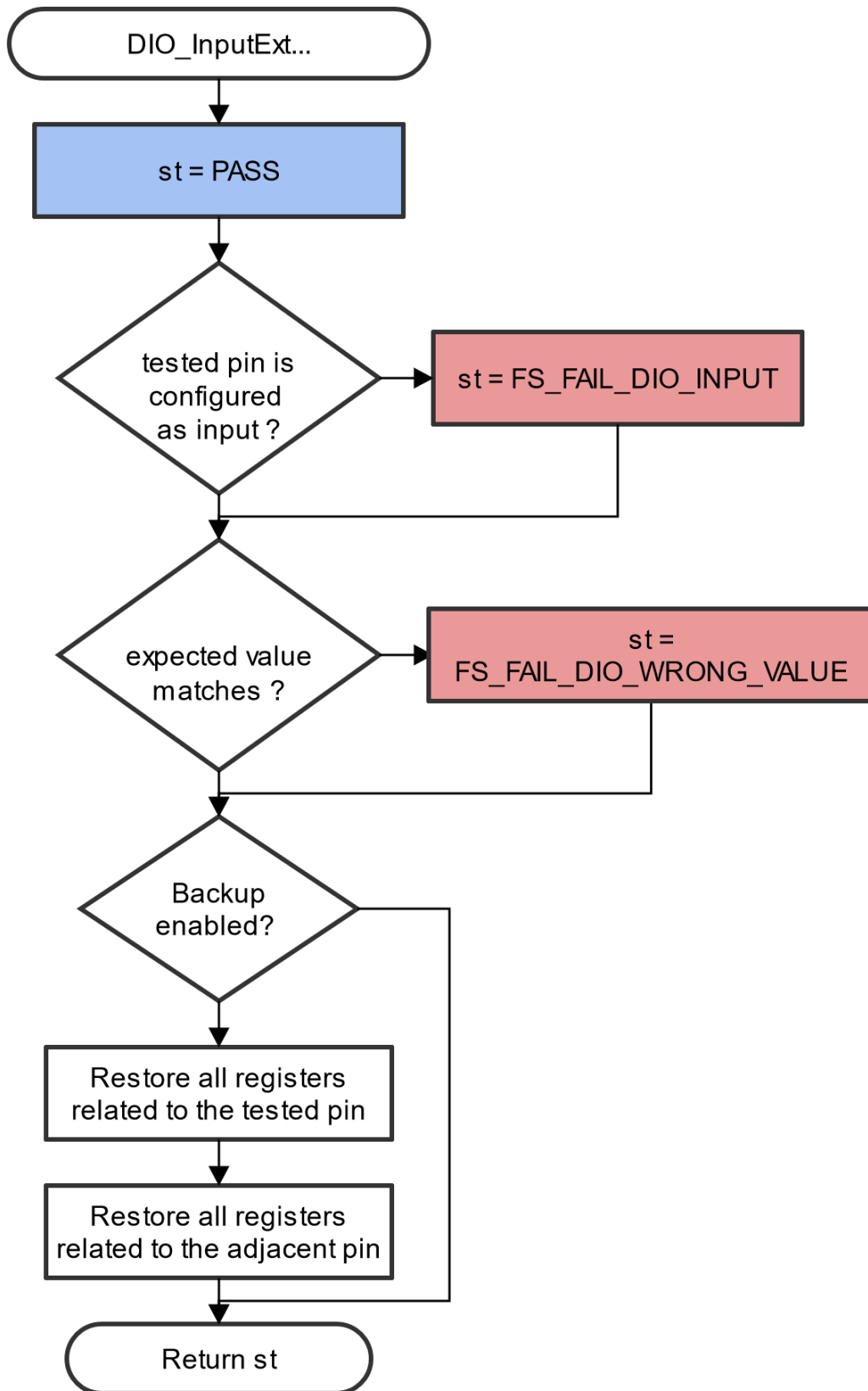
Figure 22. Extended digital input test for IMX RGPIO IEC60730_B_CM33_Library_UG_v4_3, Rev. 1, 30. September 2022
