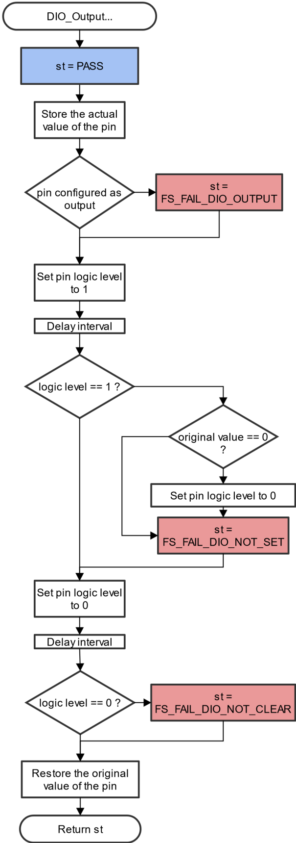
Figure 10. Block diagram for digital output test IEC60730_B_CM33_Library_UG_v4_3, Rev. 1, 30. September 2022
