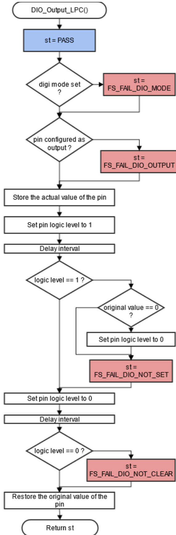
Figure 19. Block diagram for digital output test IEC60730-B_CM33_Library_UG_v4_3, Rev. 1, 30. September 2022
