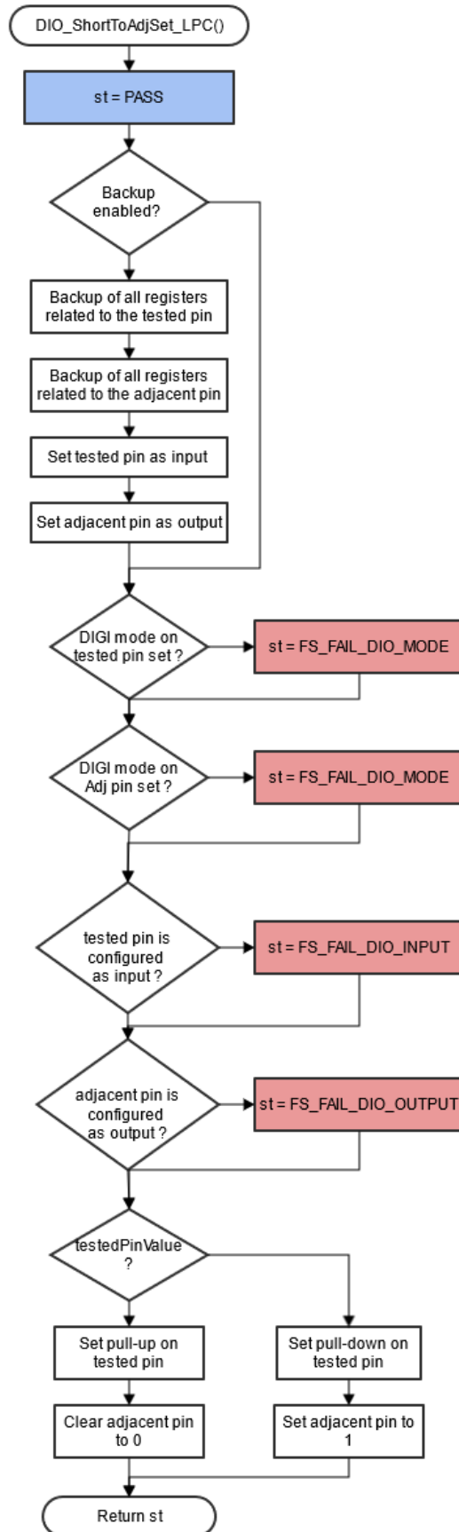
Figure 20. Block diagram of FS_DIO_ShortToAdjSet_LPC() function IEC60730_B_CM33_Library_UG_v4_3, Rev. 1, 30. September 2022
