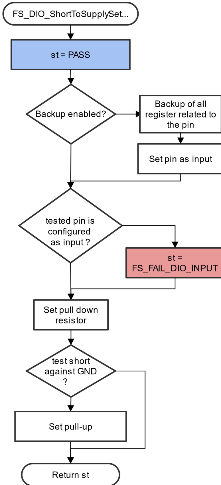
Figure 17. Block diagram of FS_DIO_ShortToSupplySet_IMXRT() function IEC60730_B_CM33_Library_UG_v4_3, Rev. 1, 30. September 2022
