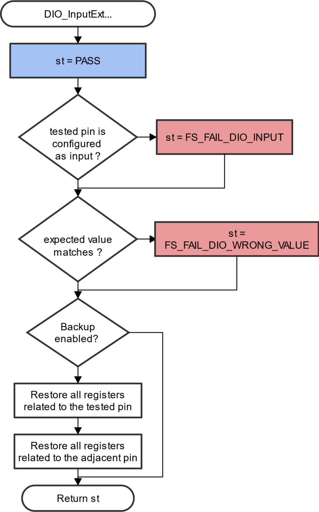
Figure 14. Extended digital input test for IMXRT IEC60730_B_CM33_Library_UG_v4_3, Rev. 1, 30. September 2022
