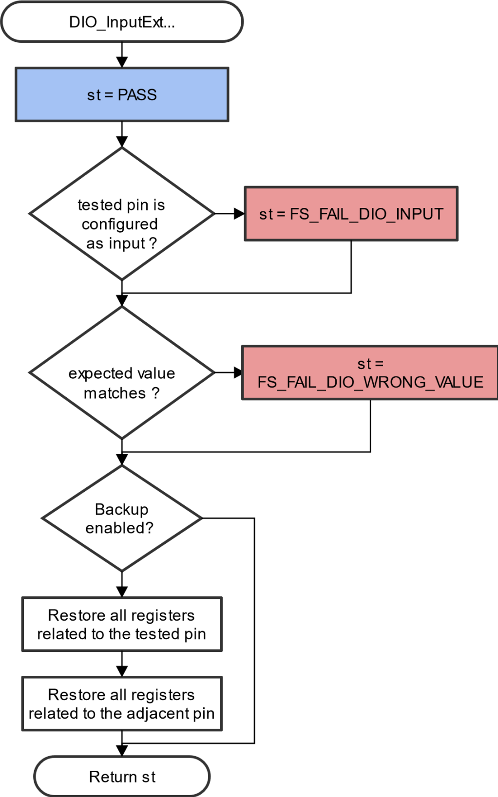
Figure 9. Extended digital input test for IMX8M IEC60730_B_CM33_Library_UG_v4_3, Rev. 1, 30. September 2022
