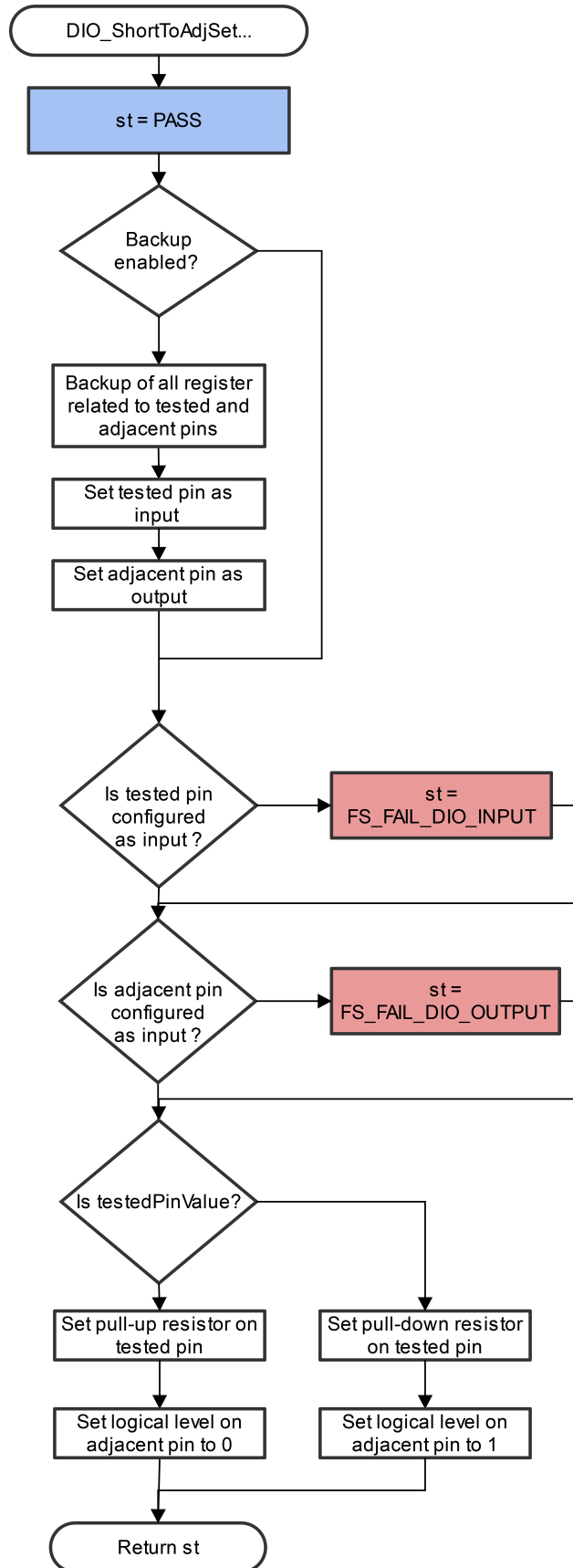
Figure 11. Block diagram of FS_DIO_ShortToAdjSet_IMX8M0 function IEC60730_B_CM33_Library_UG_v4_3, Rev. 1, 30. September 2022
