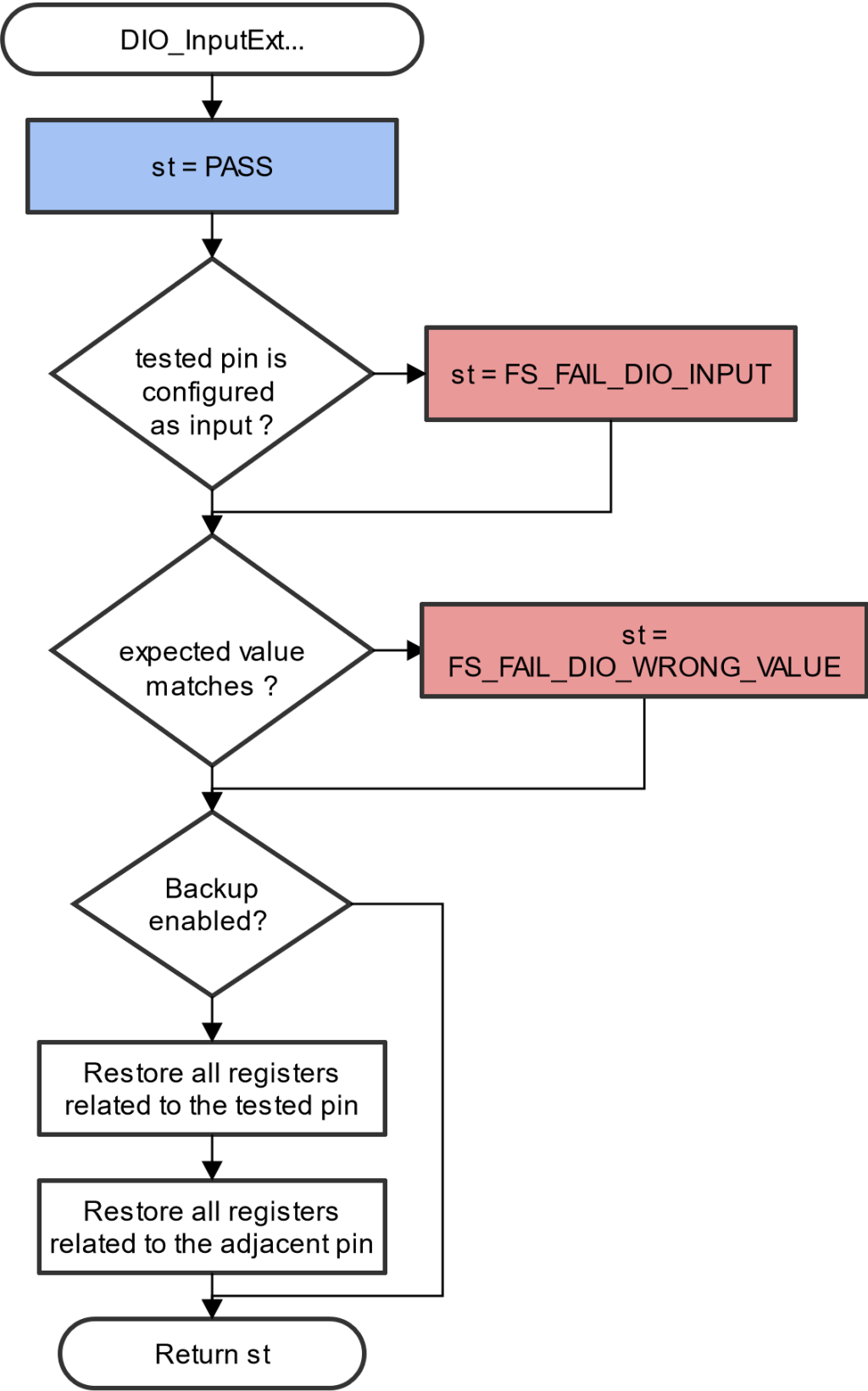
Figure 6. Extended digital input test IEC60730_B_CM33_Library_UG_v4_3, Rev. 1, 30. September 2022
